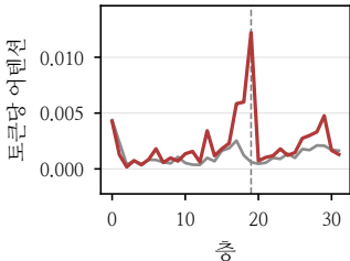
StableCode
