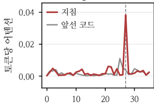
StableCode
