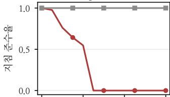
StableCode
