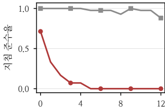
StableCode
