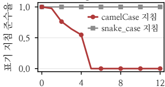
Qwen2.5
