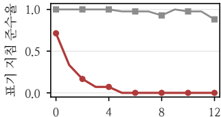
StableCode
