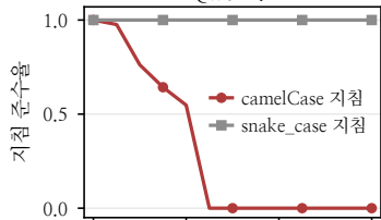
Qwen2.5
