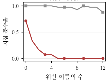
StableCode
