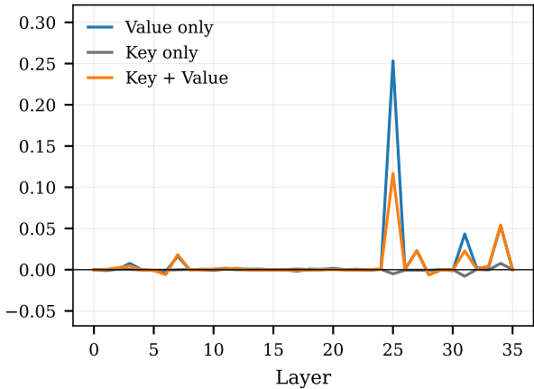
Notation-specific recovery
