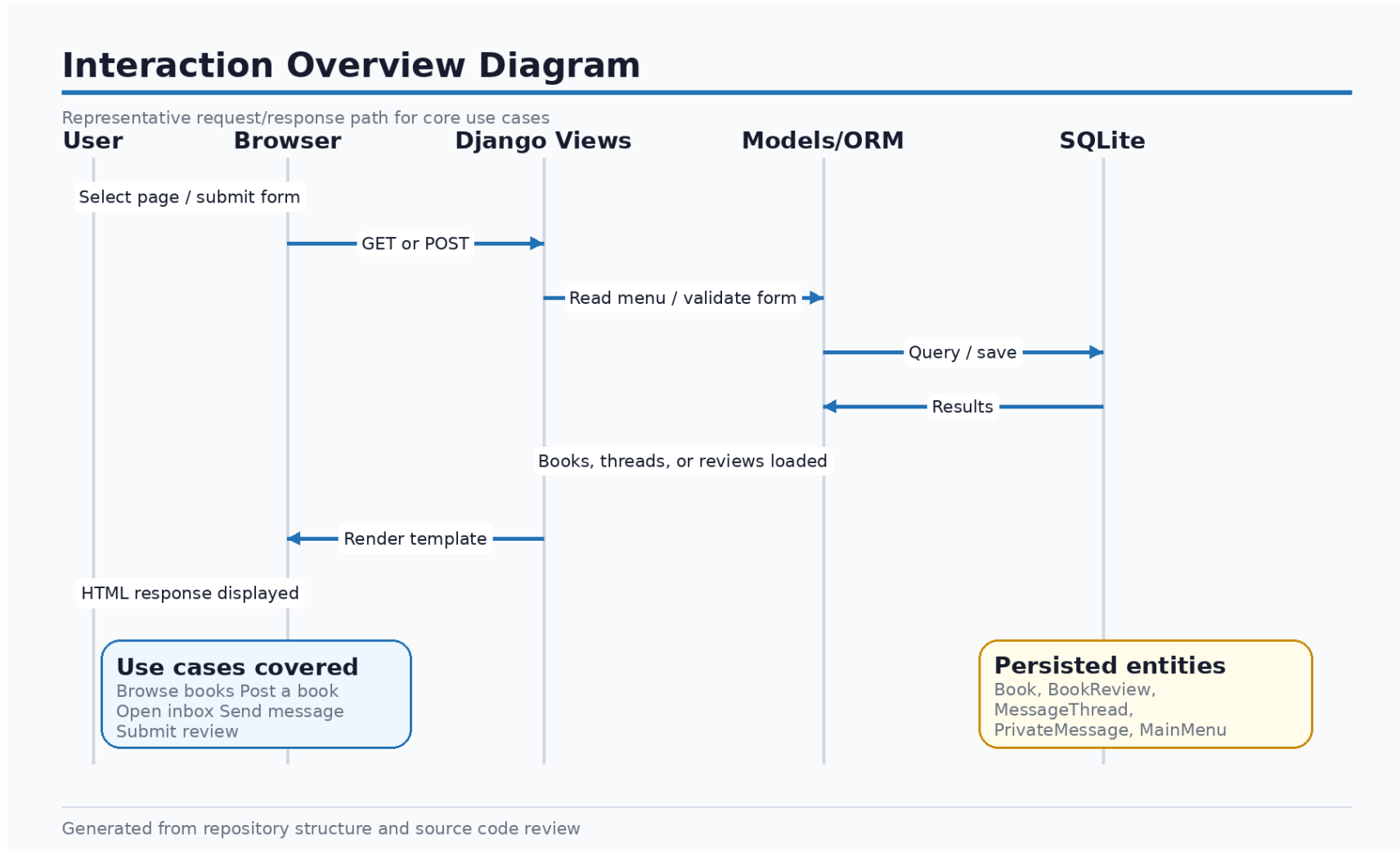
Figure: 3. Design Document - Interaction Overview Diagram
