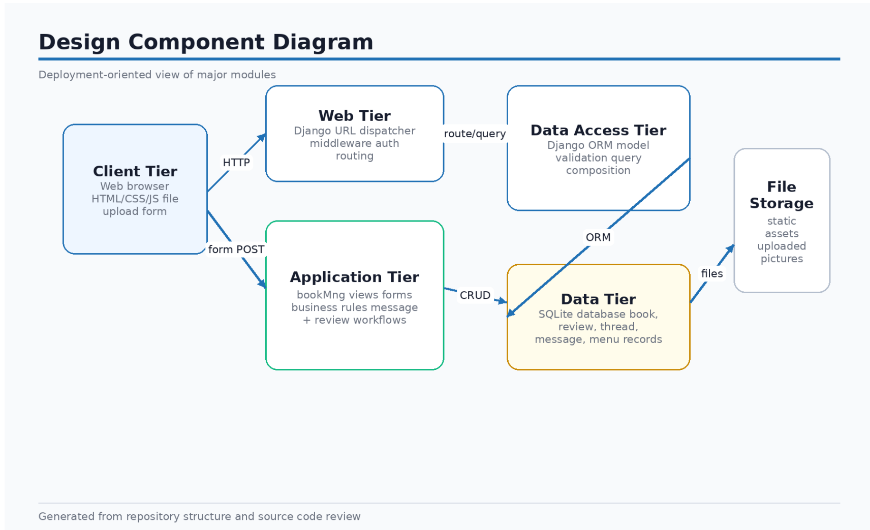
Figure: 2. Design Document - Component Diagram
