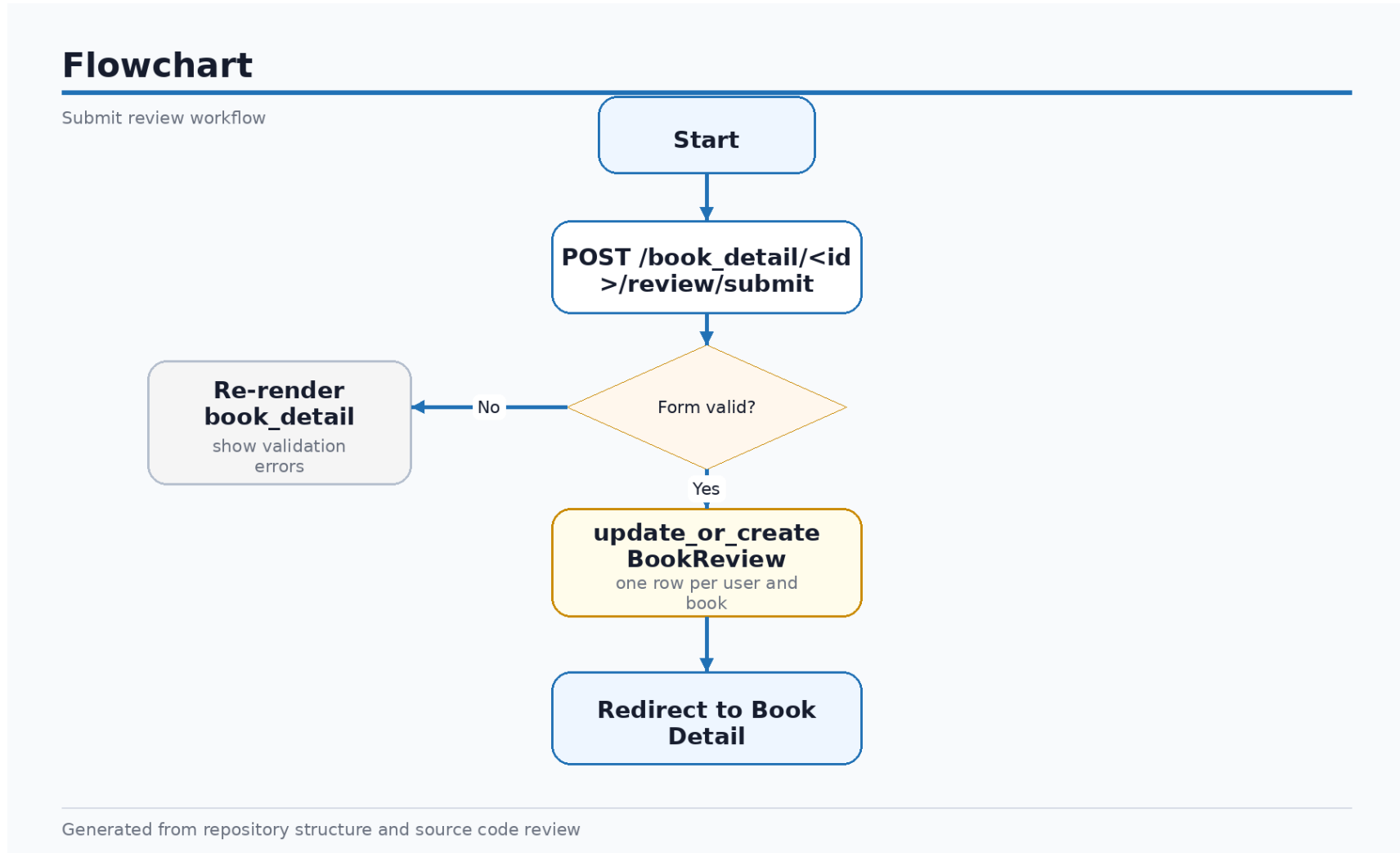
Figure: 4. Design Document - Flowchart
