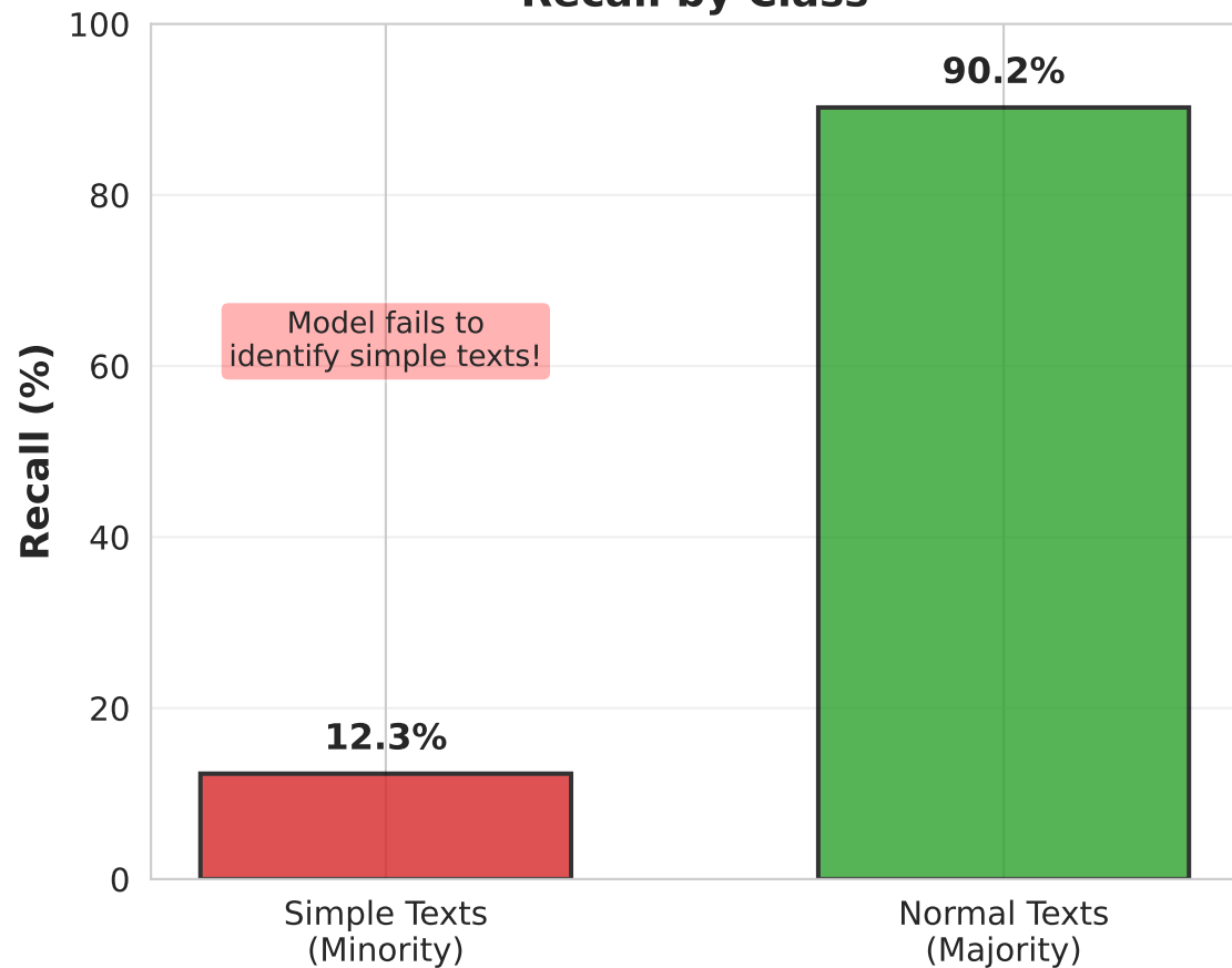
Recall by Class
