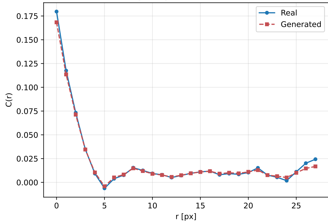
Spin-spin correlation
