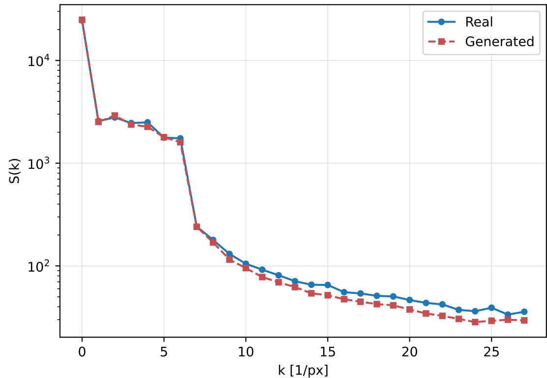
Structure factor
