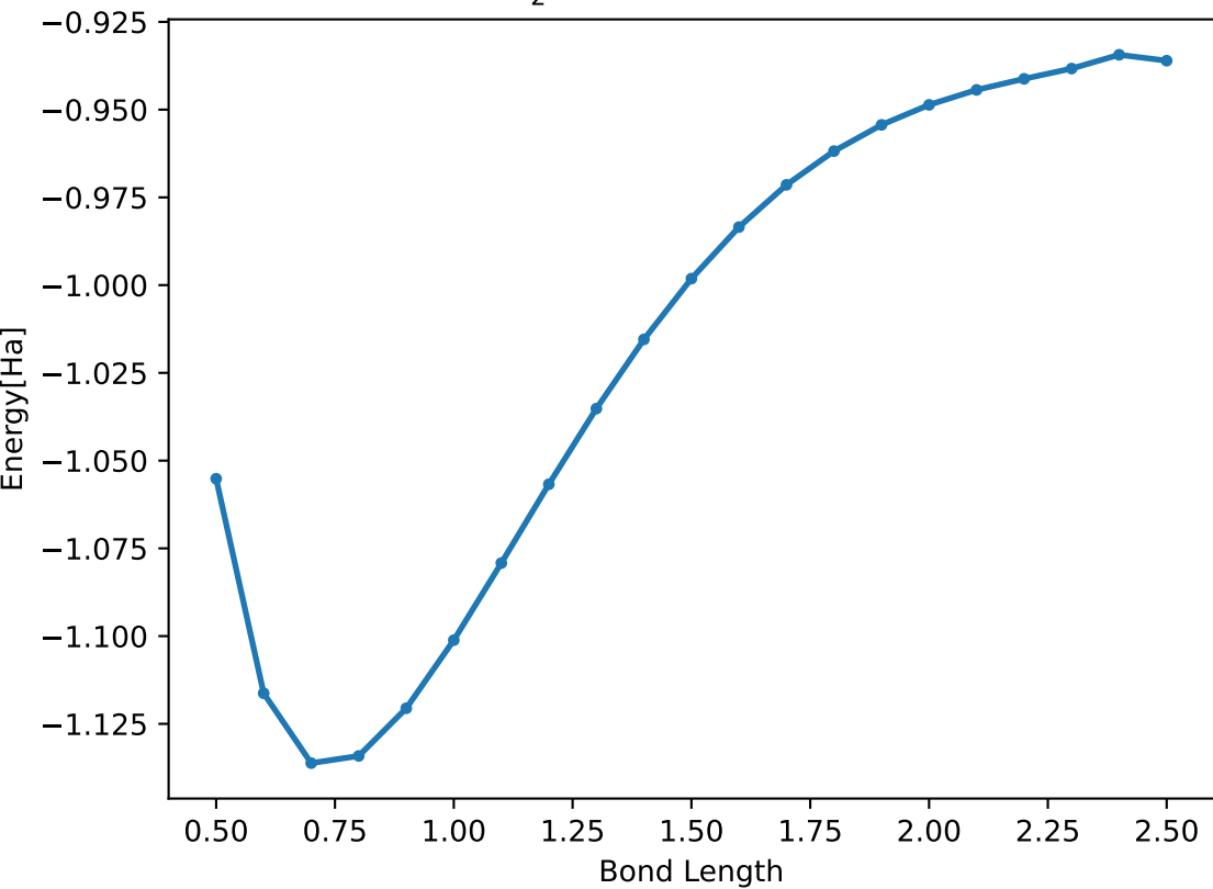
H_2 dissociation curve
