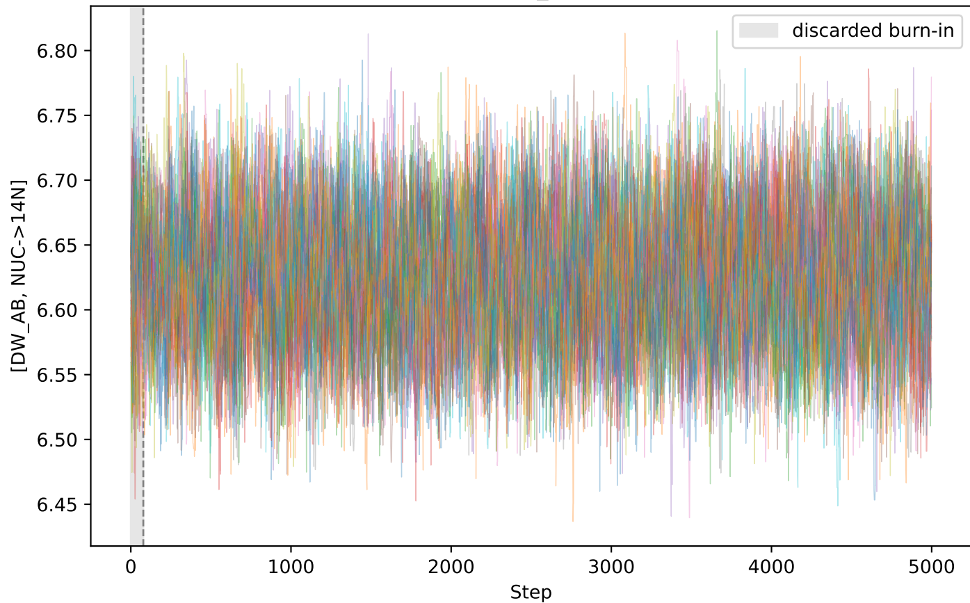
MCMC trace: [DW_AB, NUC->14N]
