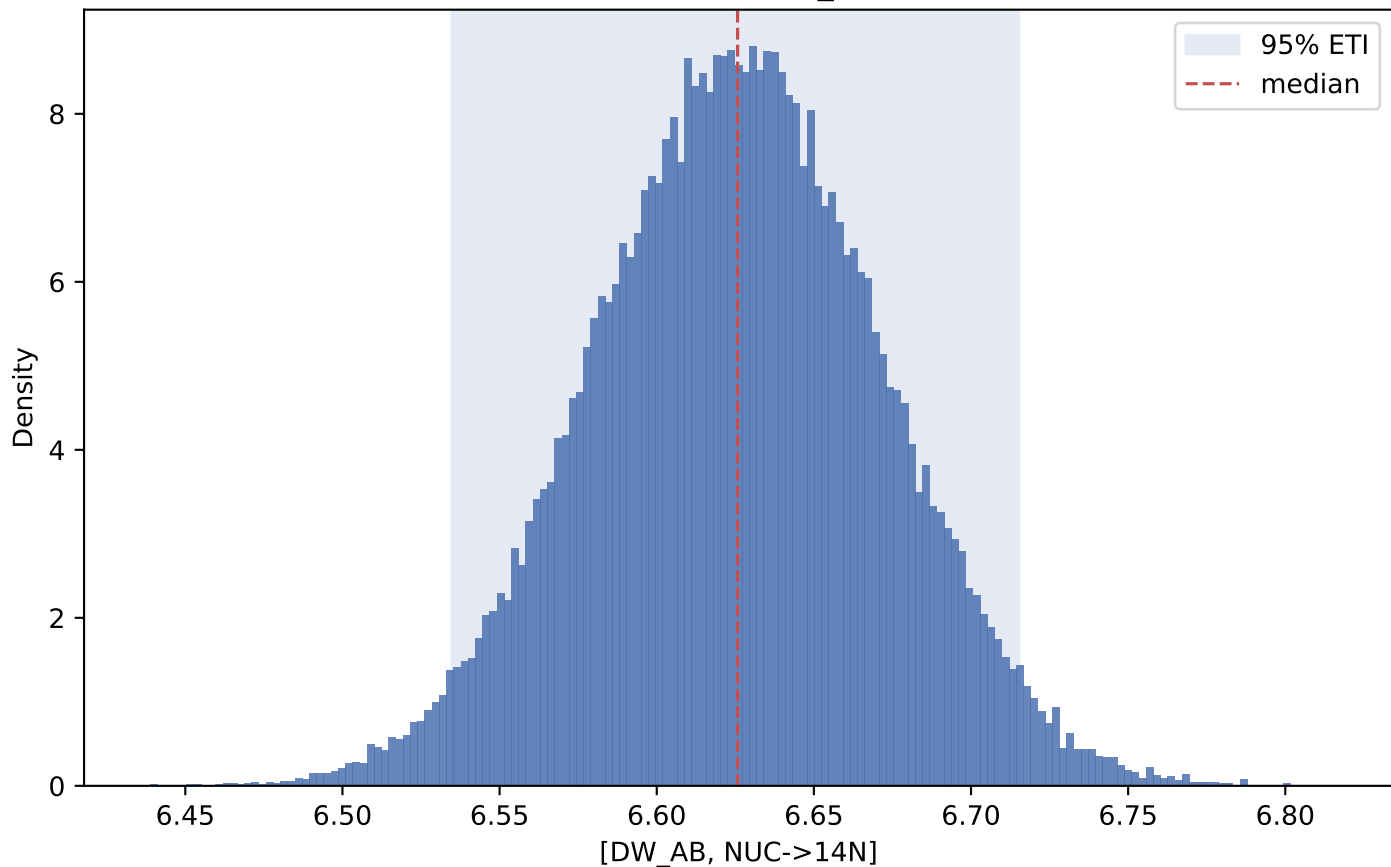
Posterior distribution: [DW_AB, NUC->14N]
