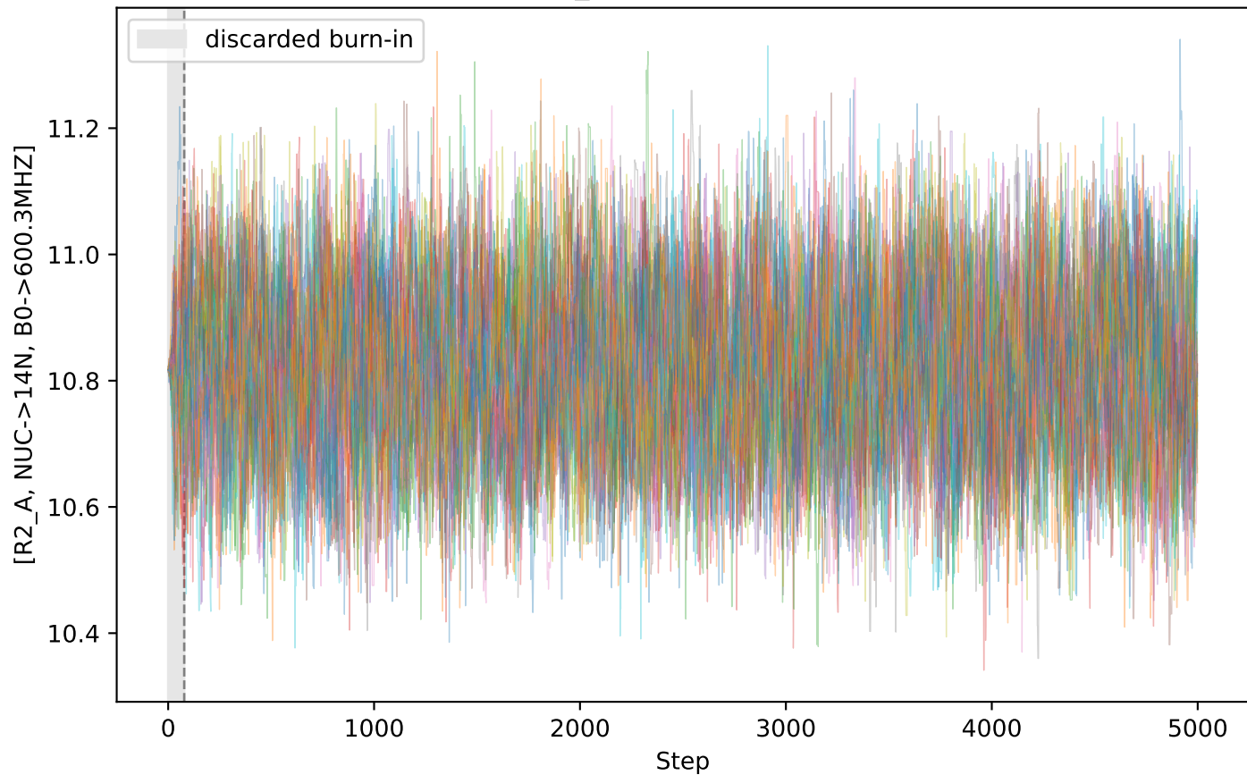
MCMC trace: [R2_A, NUC->14N, B0->600.3MHZ]
