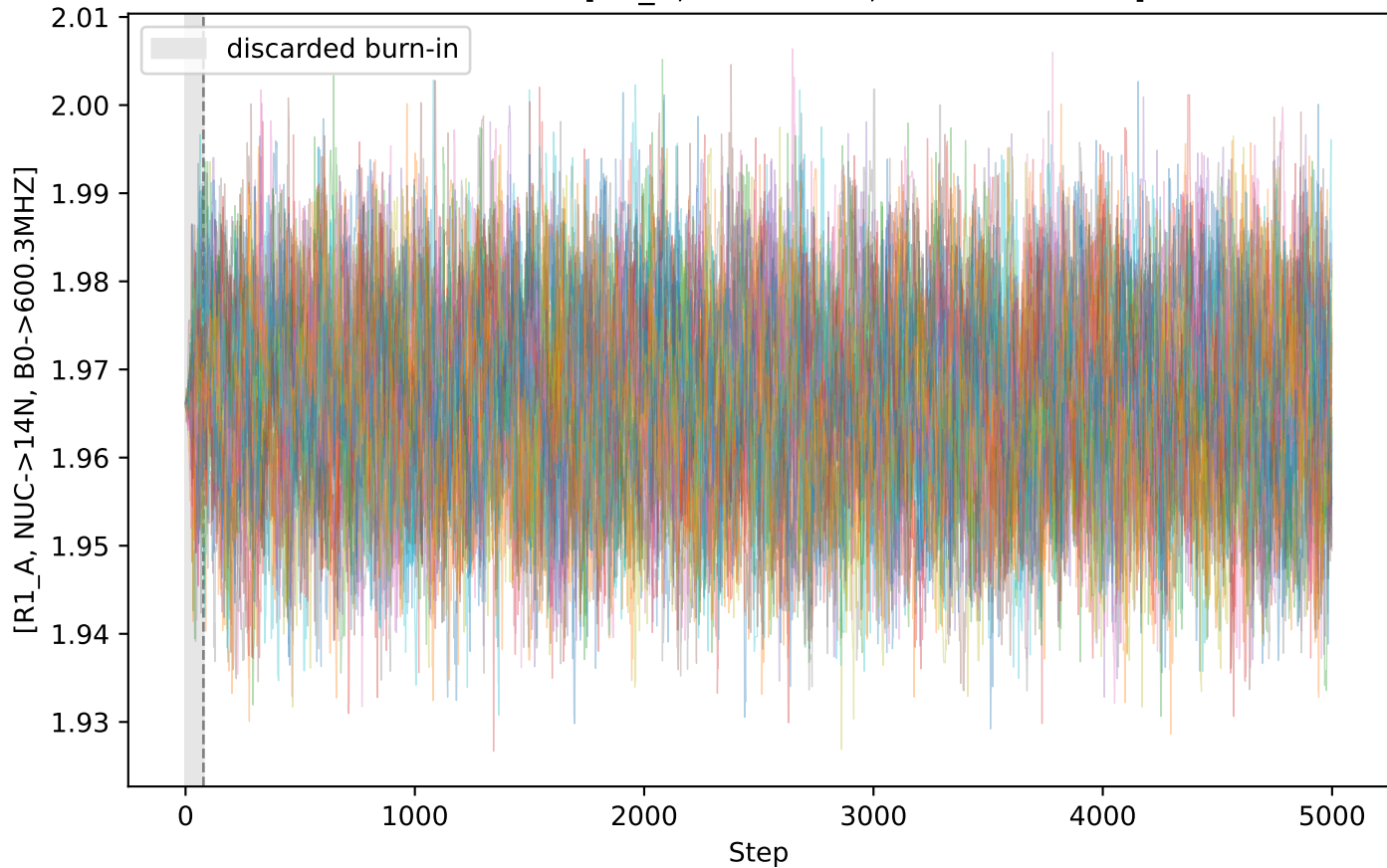
MCMC trace: [R1_A, NUC->14N, B0->600.3MHZ]
