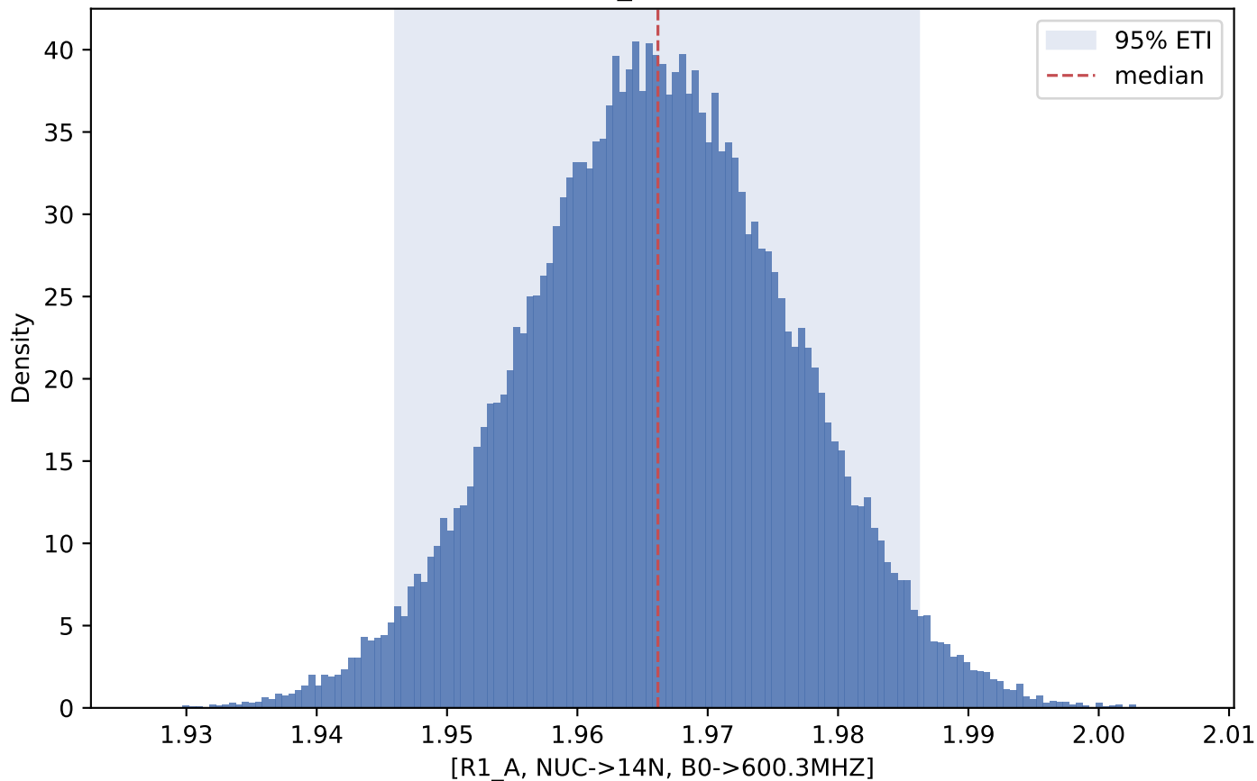
Posterior distribution: [R1_A, NUC->14N, B0->600.3MHZ]
