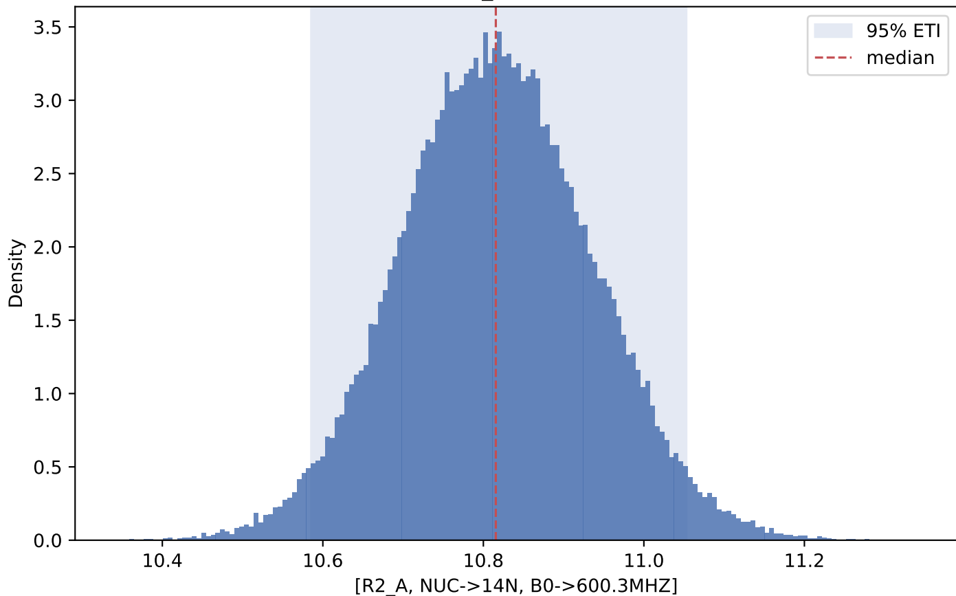
Posterior distribution: [R2_A, NUC->14N, B0->600.3MHZ]
