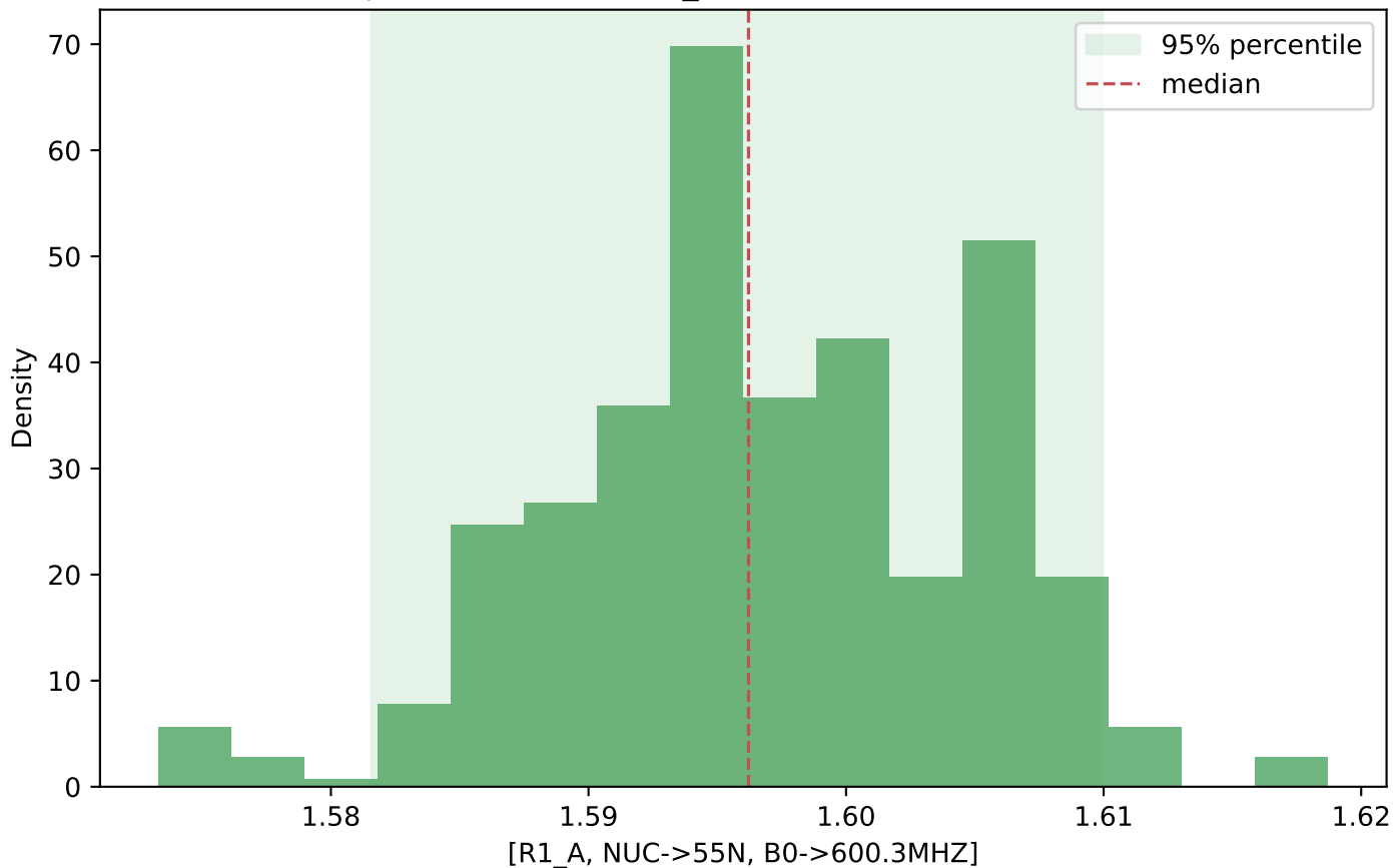
Sample distribution: [R1_A, NUC->55N, B0->600.3MHZ]
