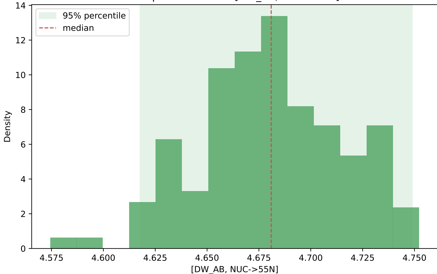
Sample distribution: [DW_AB, NUC->55N]
