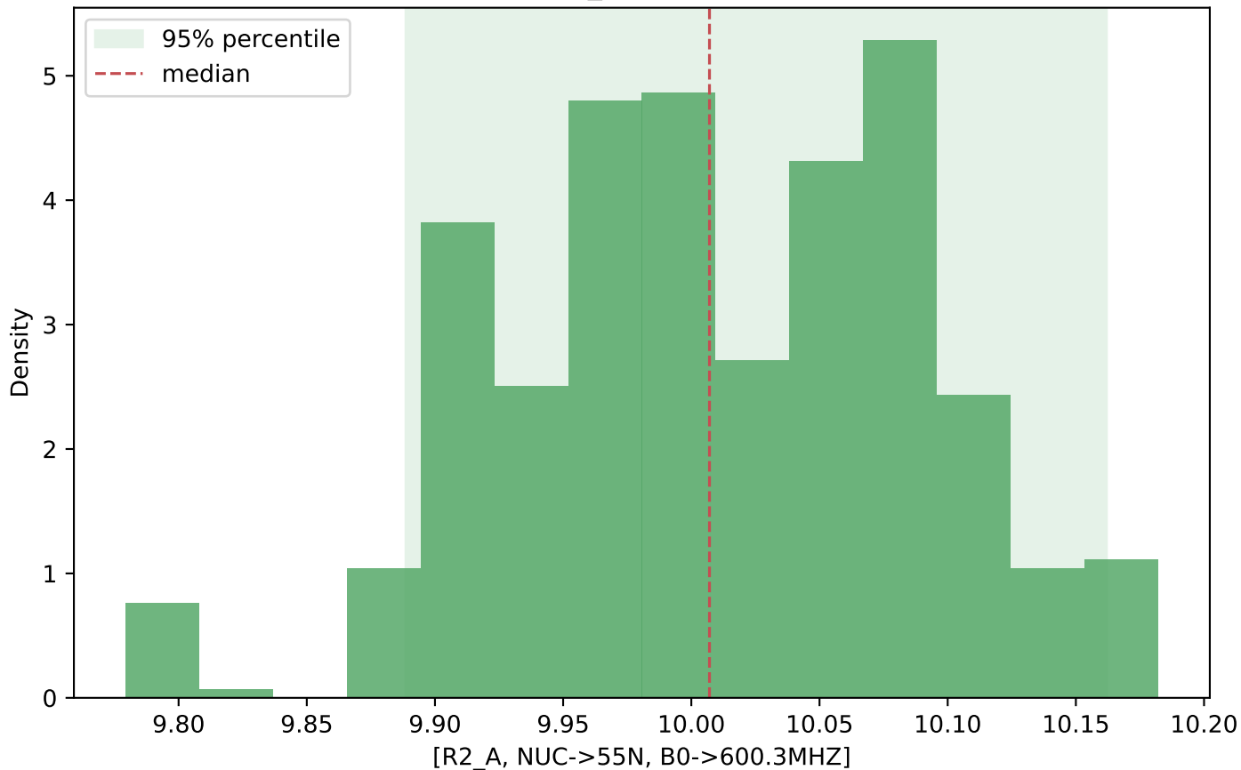
Sample distribution: [R2_A, NUC->55N, B0->600.3MHZ]
