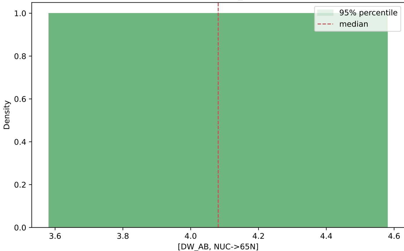
Sample distribution: [DW_AB, NUC->65N]
