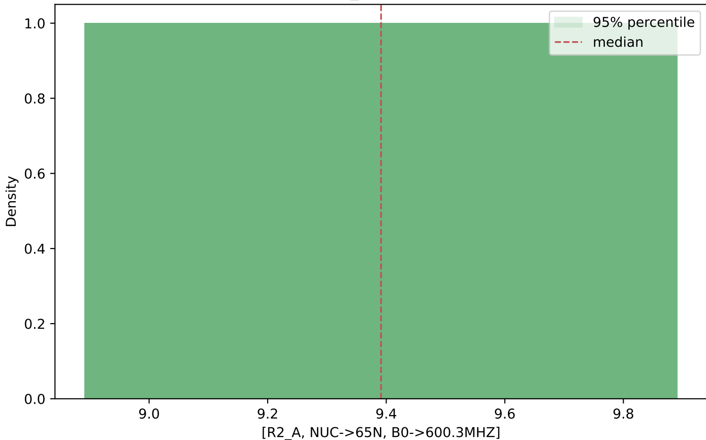
Sample distribution: [R2_A, NUC->65N, B0->600.3MHZ]
