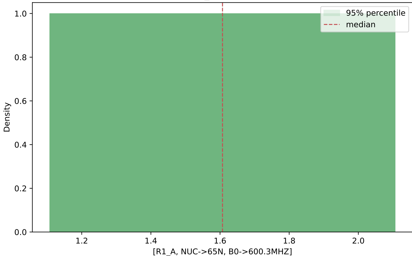
Sample distribution: [R1_A, NUC->65N, B0->600.3MHZ]
