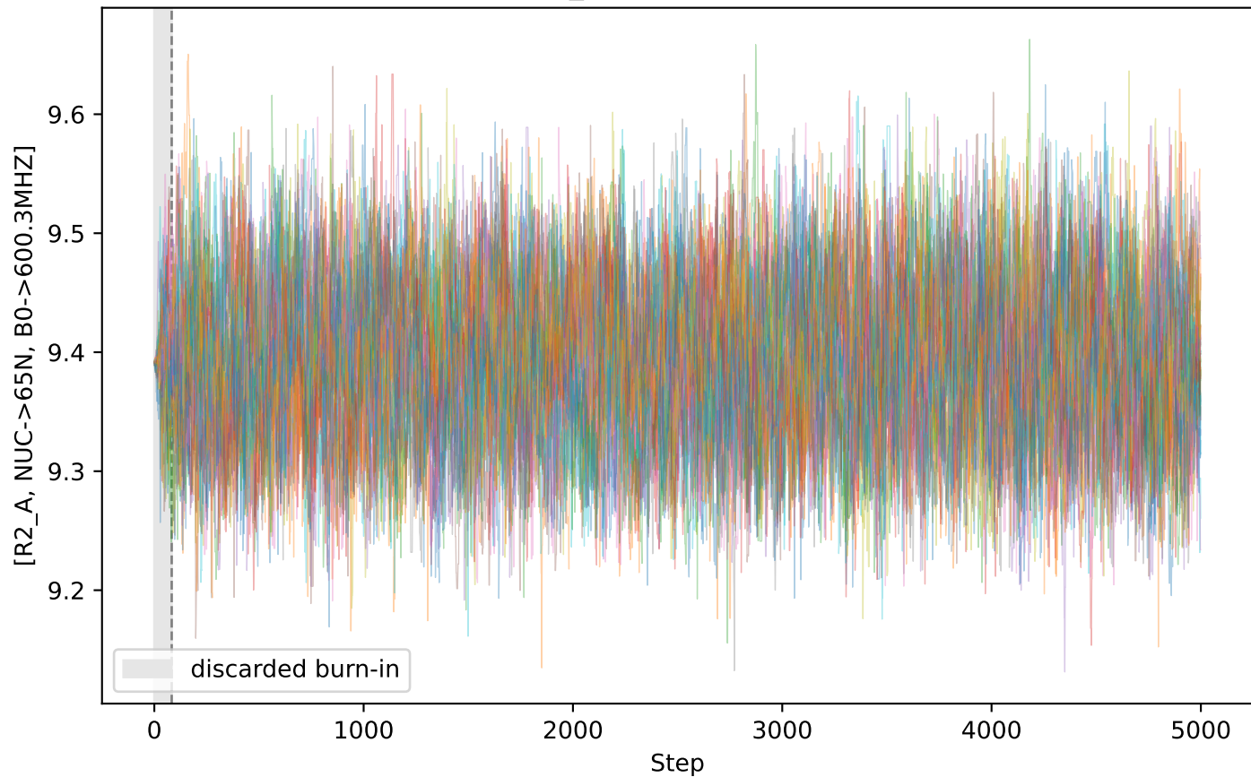
MCMC trace: [R2_A, NUC->65N, B0->600.3MHZ]
