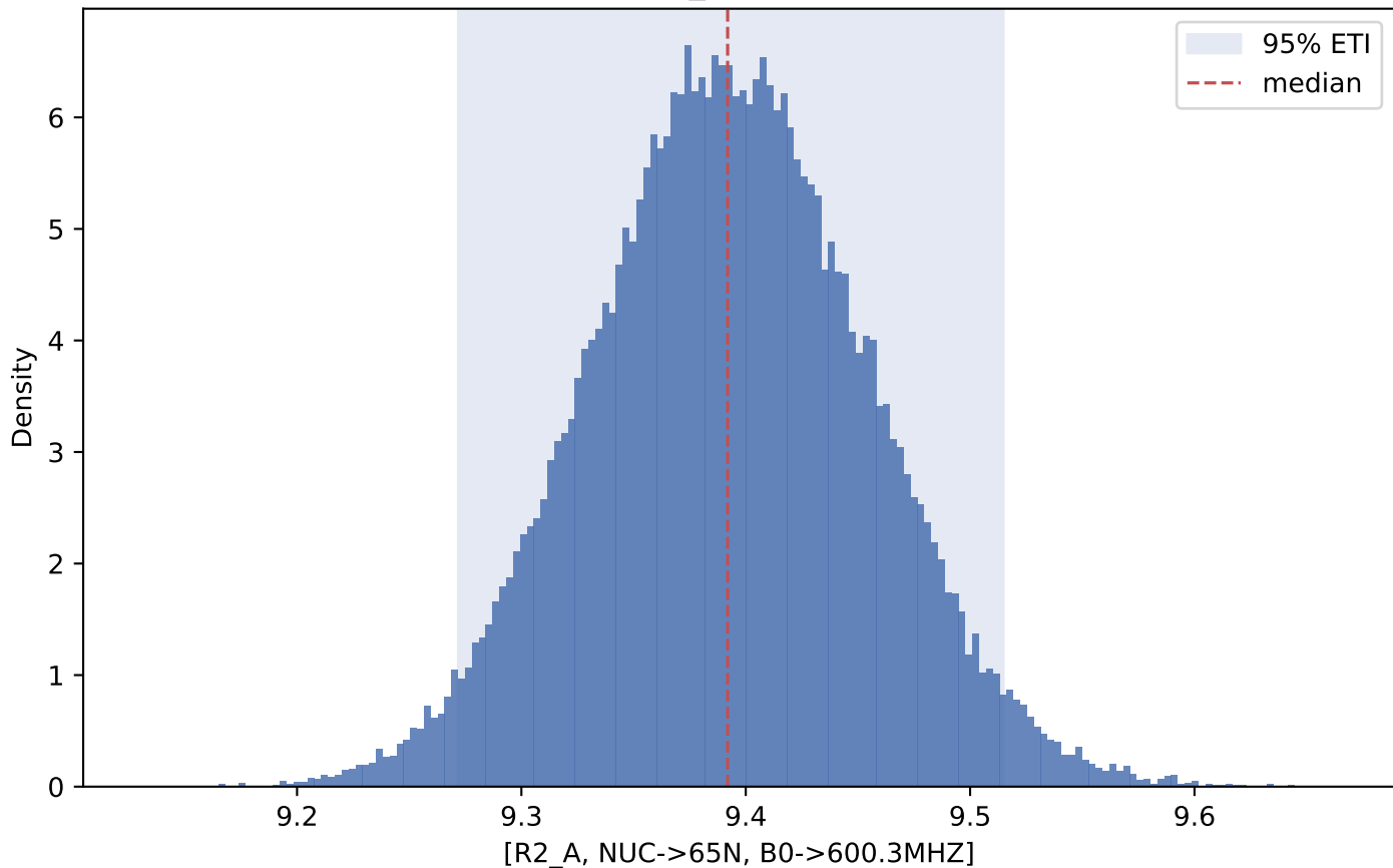
Posterior distribution: [R2_A, NUC->65N, B0->600.3MHZ]
