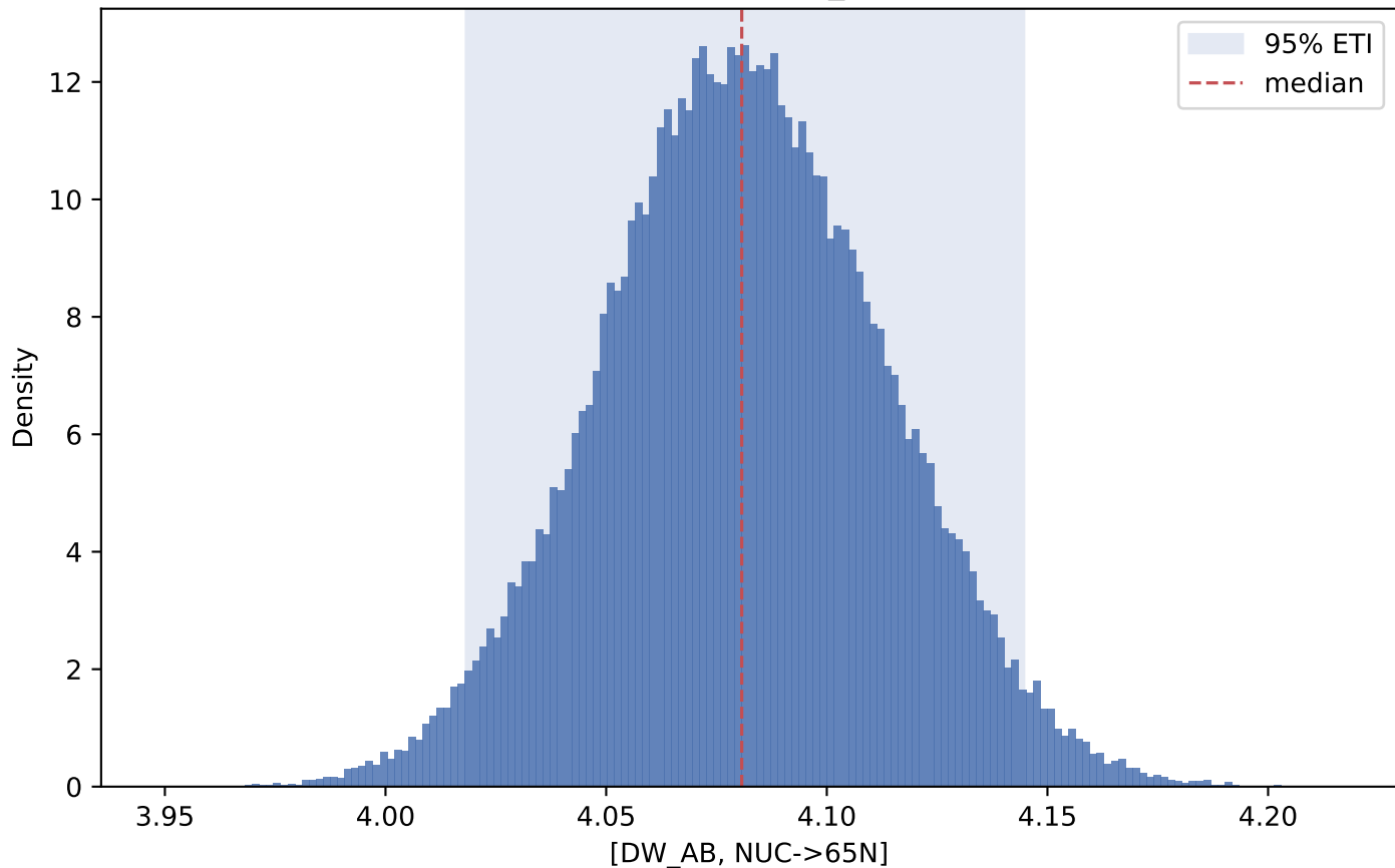
Posterior distribution: [DW_AB, NUC->65N]
