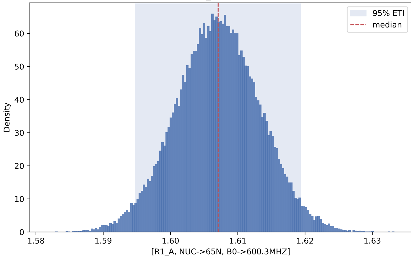
Posterior distribution: [R1_A, NUC->65N, B0->600.3MHZ]
