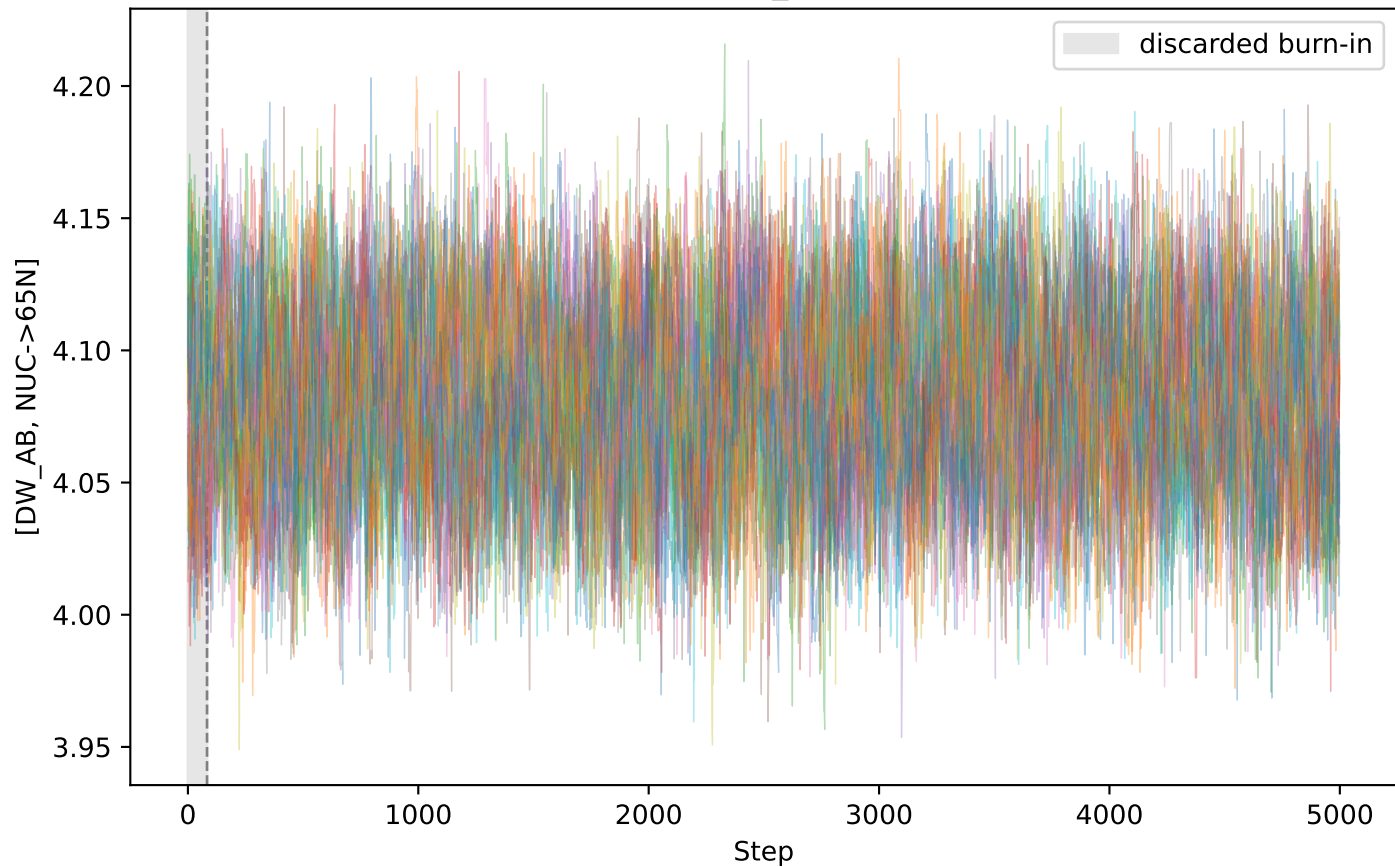
MCMC trace: [DW_AB, NUC->65N]
