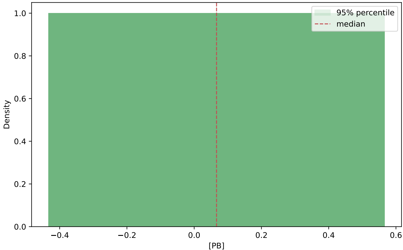
Sample distribution: [PB]
