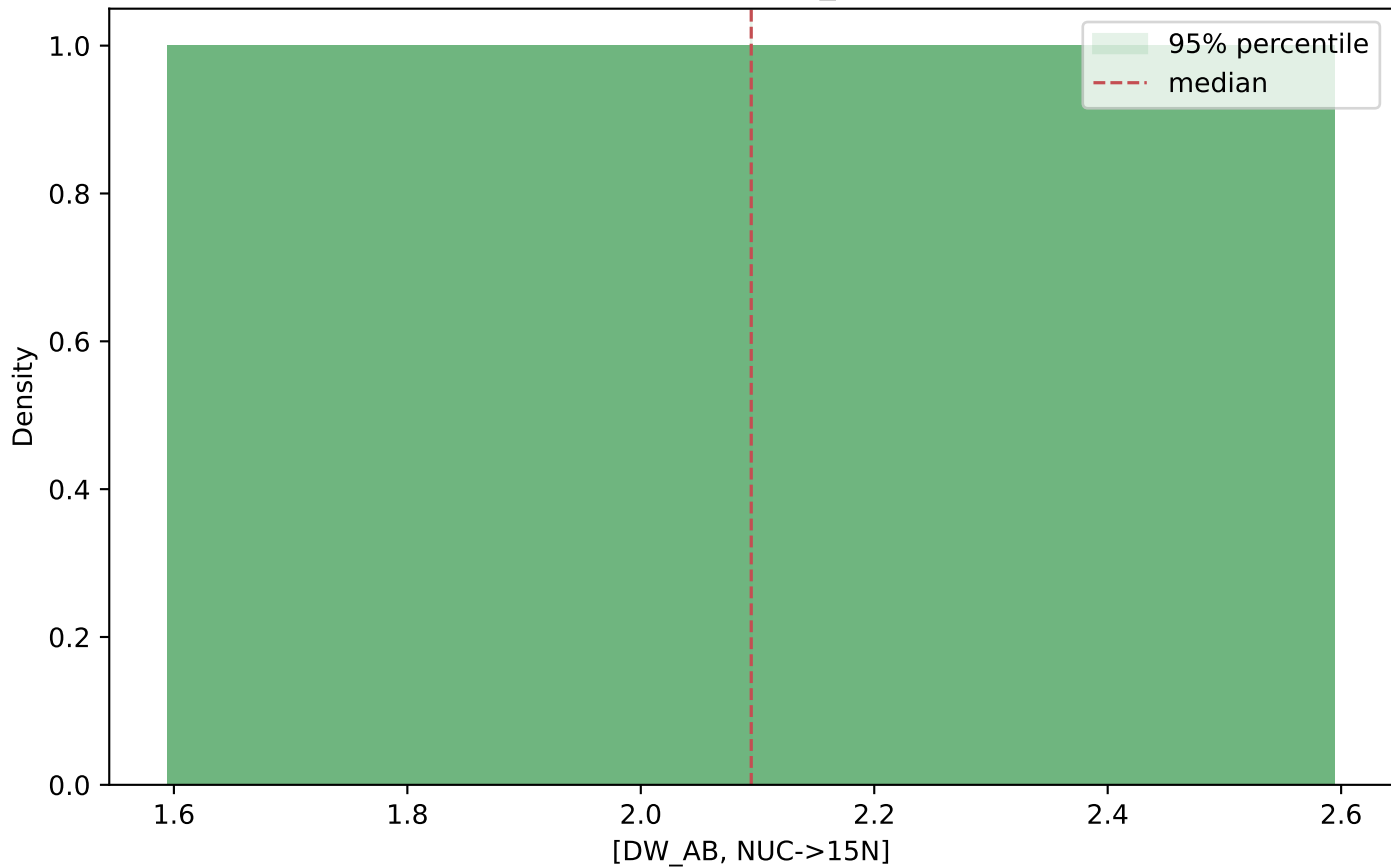
Sample distribution: [DW_AB, NUC->15N]
