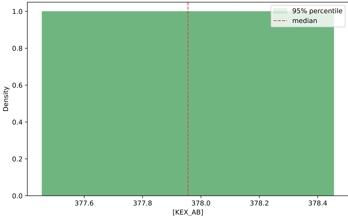
Sample distribution: [KEX_AB]
