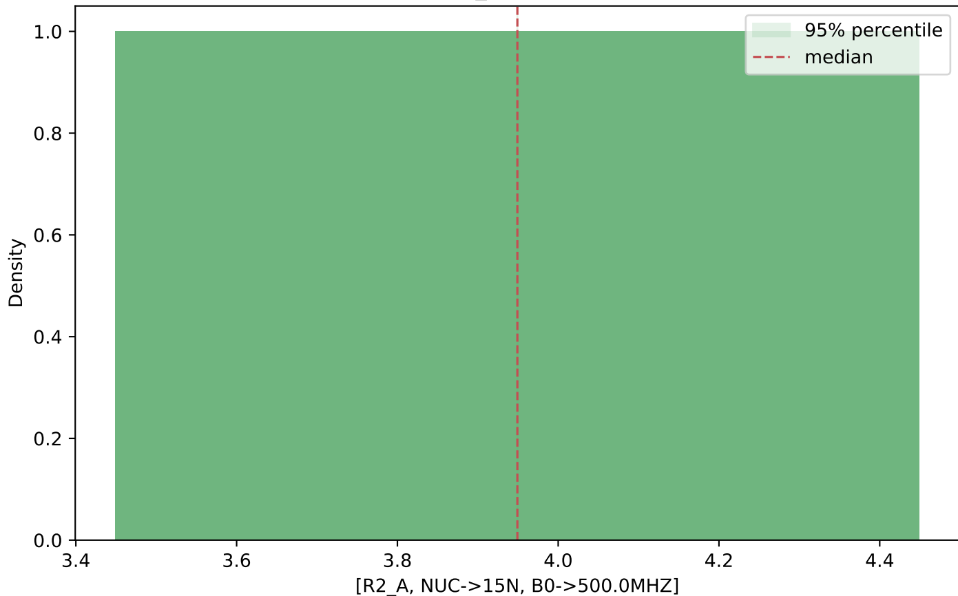
Sample distribution: [R2_A, NUC->15N, B0->500.0MHZ]
