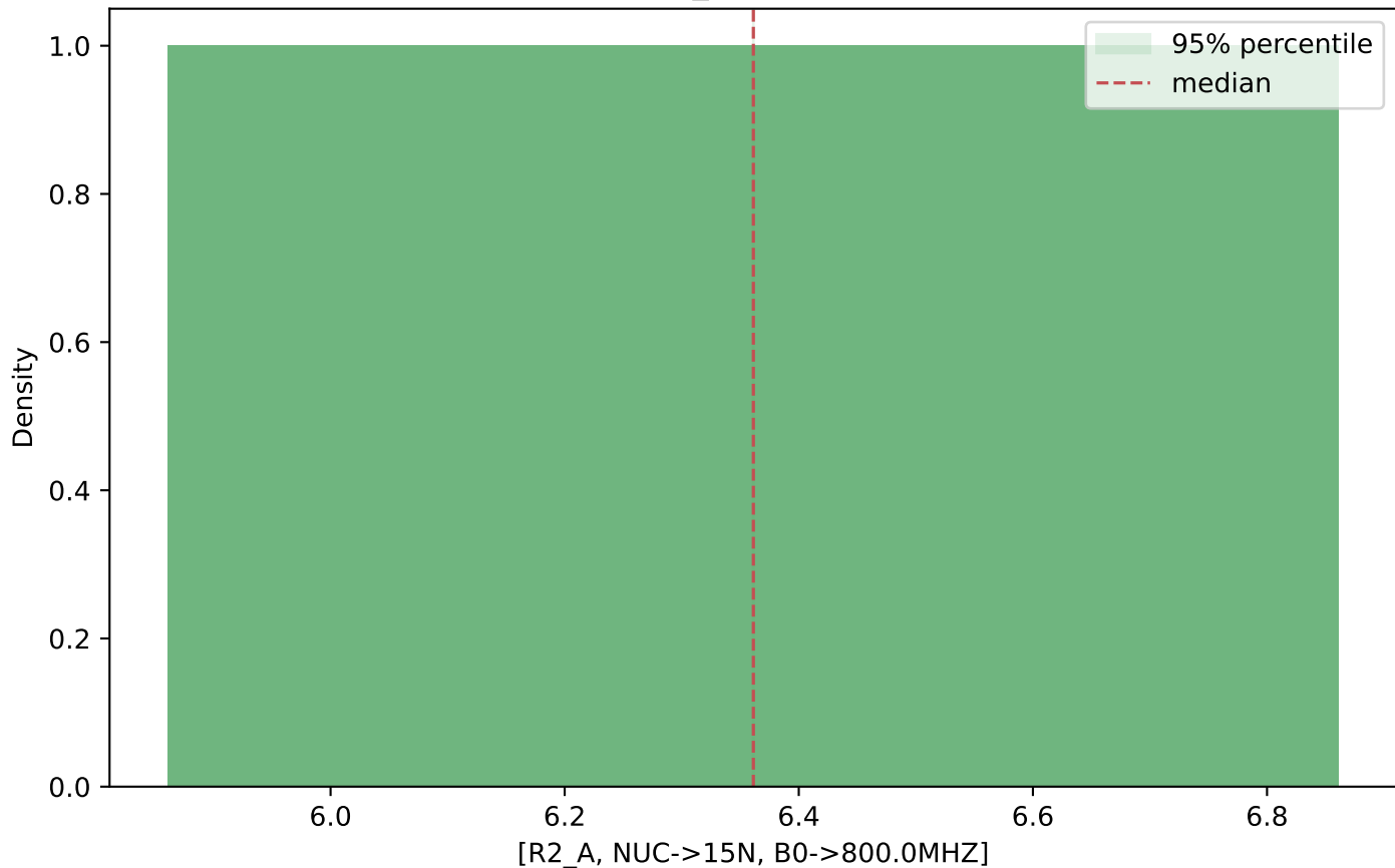
Sample distribution: [R2_A, NUC->15N, B0->800.0MHZ]
