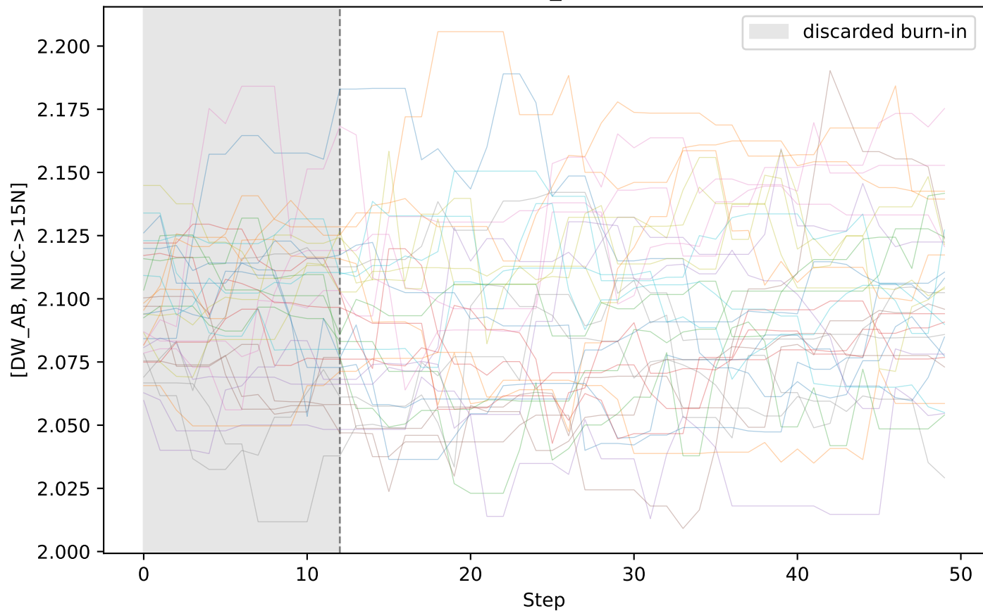
MCMC trace: [DW_AB, NUC->15N]
