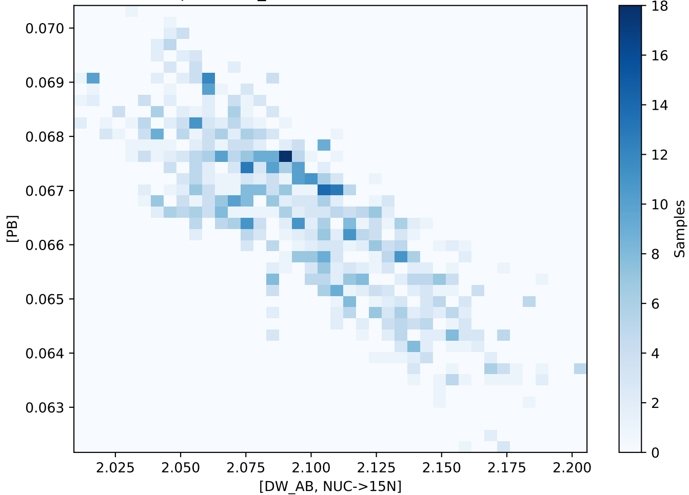
Posterior pair: [DW_AB, NUC->15N] vs [PB] ( r = -0.809 )
