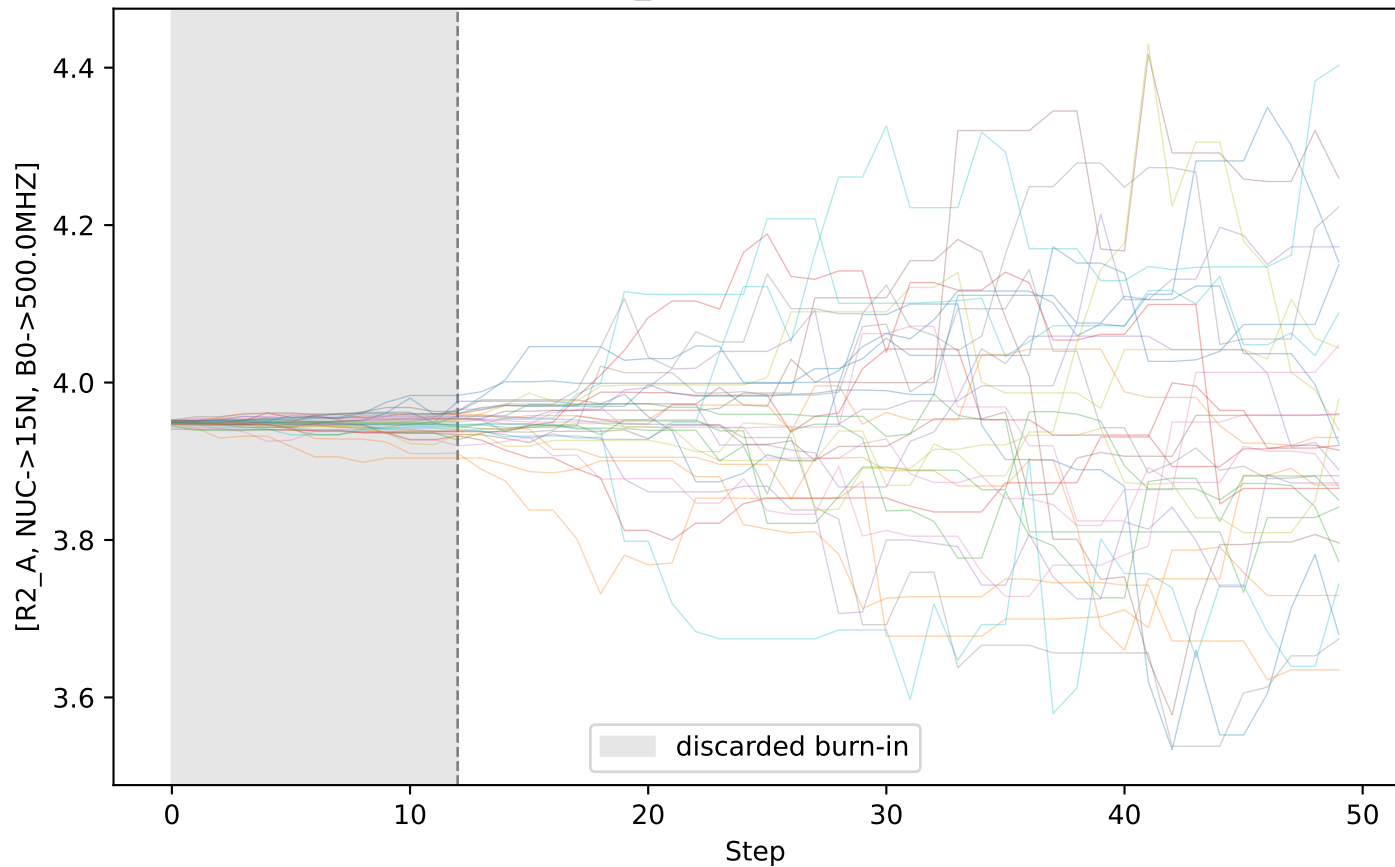
MCMC trace: [R2_A, NUC->15N, B0->500.0MHZ]
