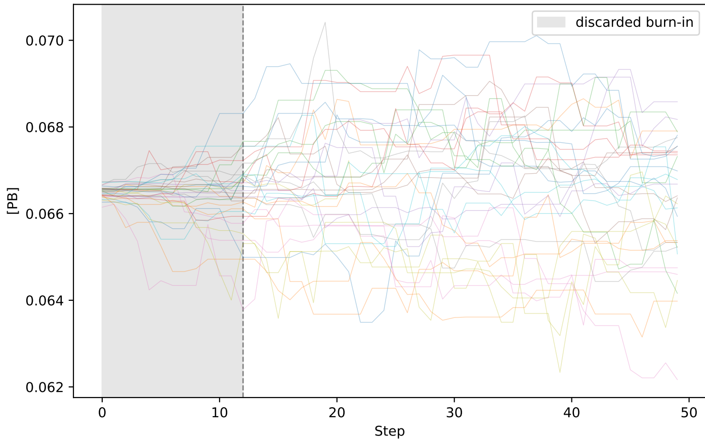
MCMC trace: [PB]
