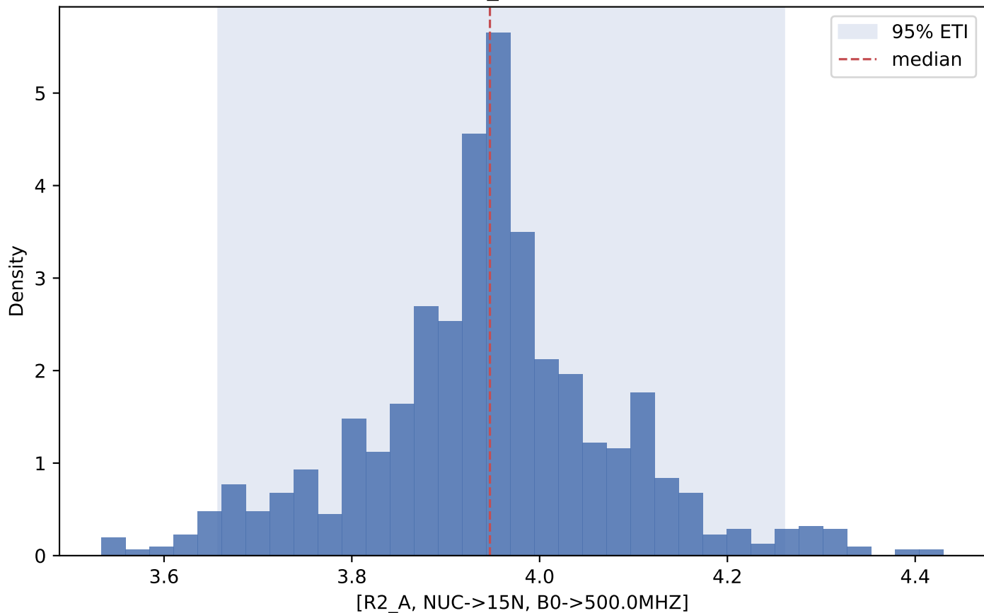
Posterior distribution: [R2_A, NUC->15N, B0->500.0MHZ]
