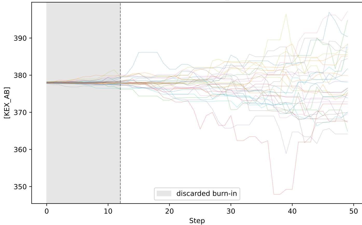
MCMC trace: [KEX_AB]
