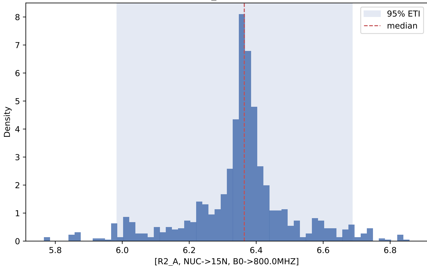
Posterior distribution: [R2_A, NUC->15N, B0->800.0MHZ]
