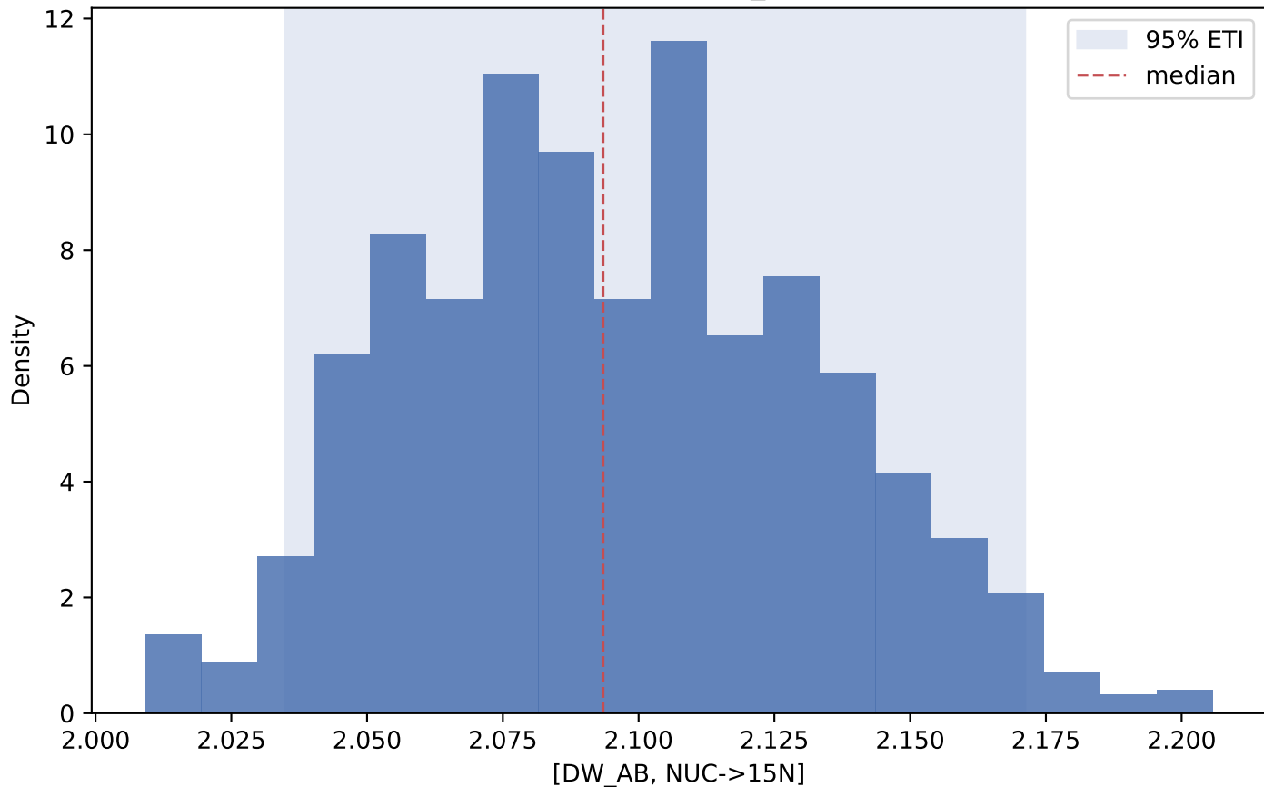
Posterior distribution: [DW_AB, NUC->15N]
