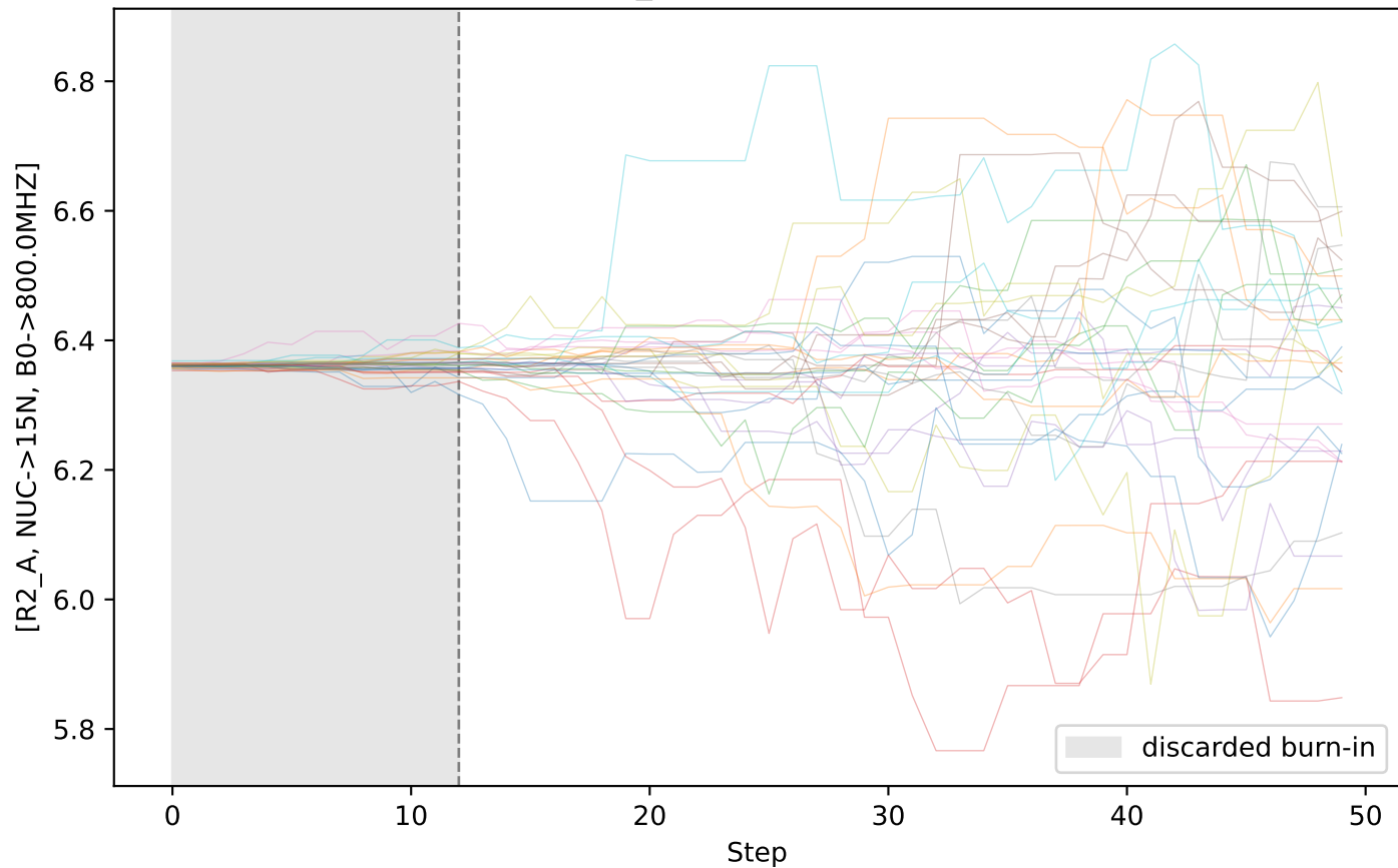
MCMC trace: [R2_A, NUC->15N, B0->800.0MHZ]
