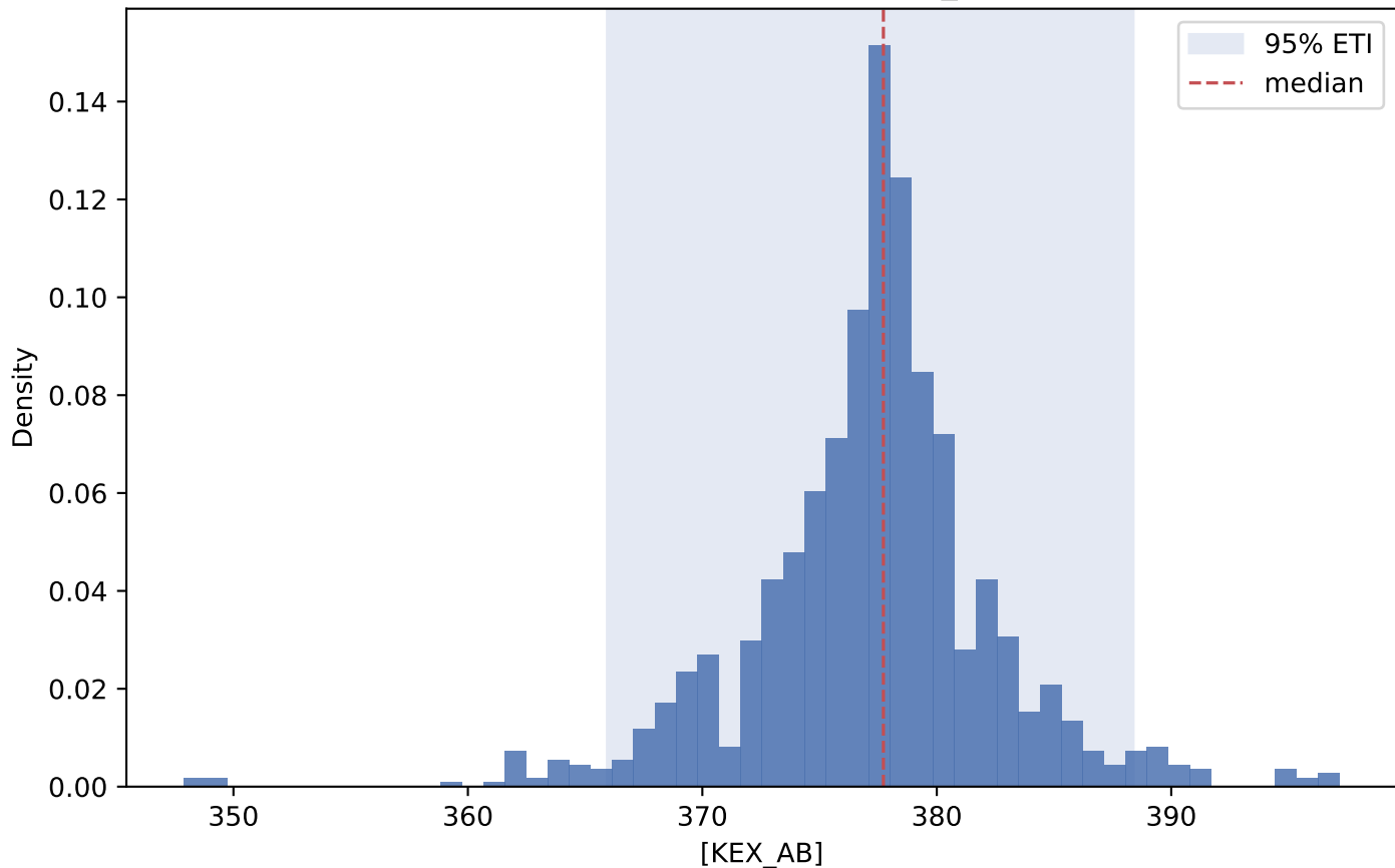
Posterior distribution: [KEX_AB]
