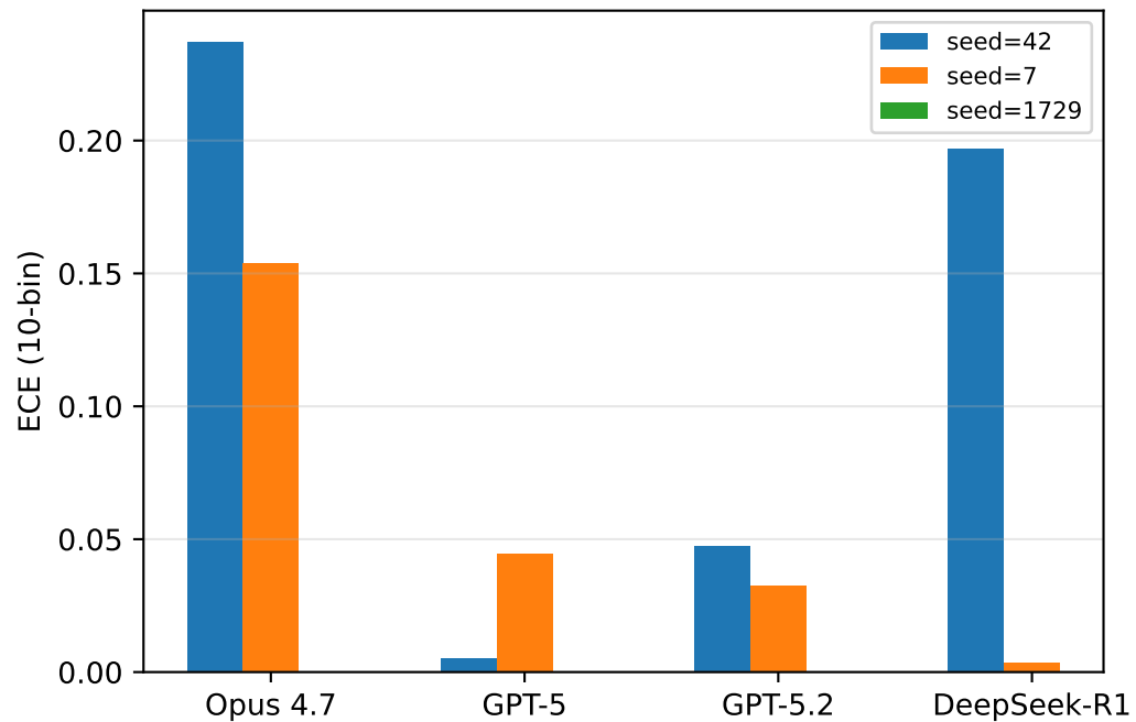
Multi-seed variance on T_extreme — Pareto-essential agents
