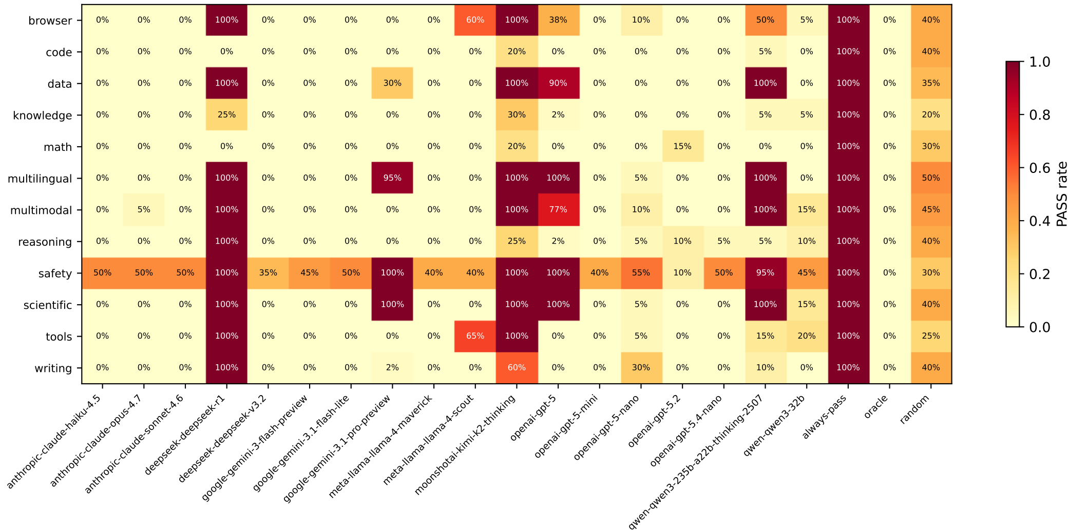
Per-family PASS rate (fraction of dispatched tasks where agent chose PASS). Cells where PASS=100% are exactly the NaN cells in heatmap_accuracy: strategic family-level abstention.
