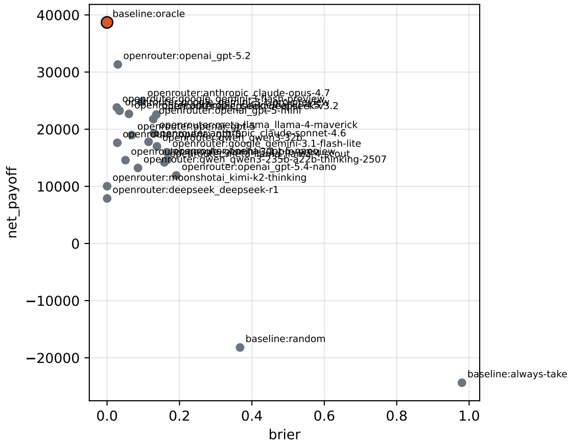
Pareto: Brier x net payoff
