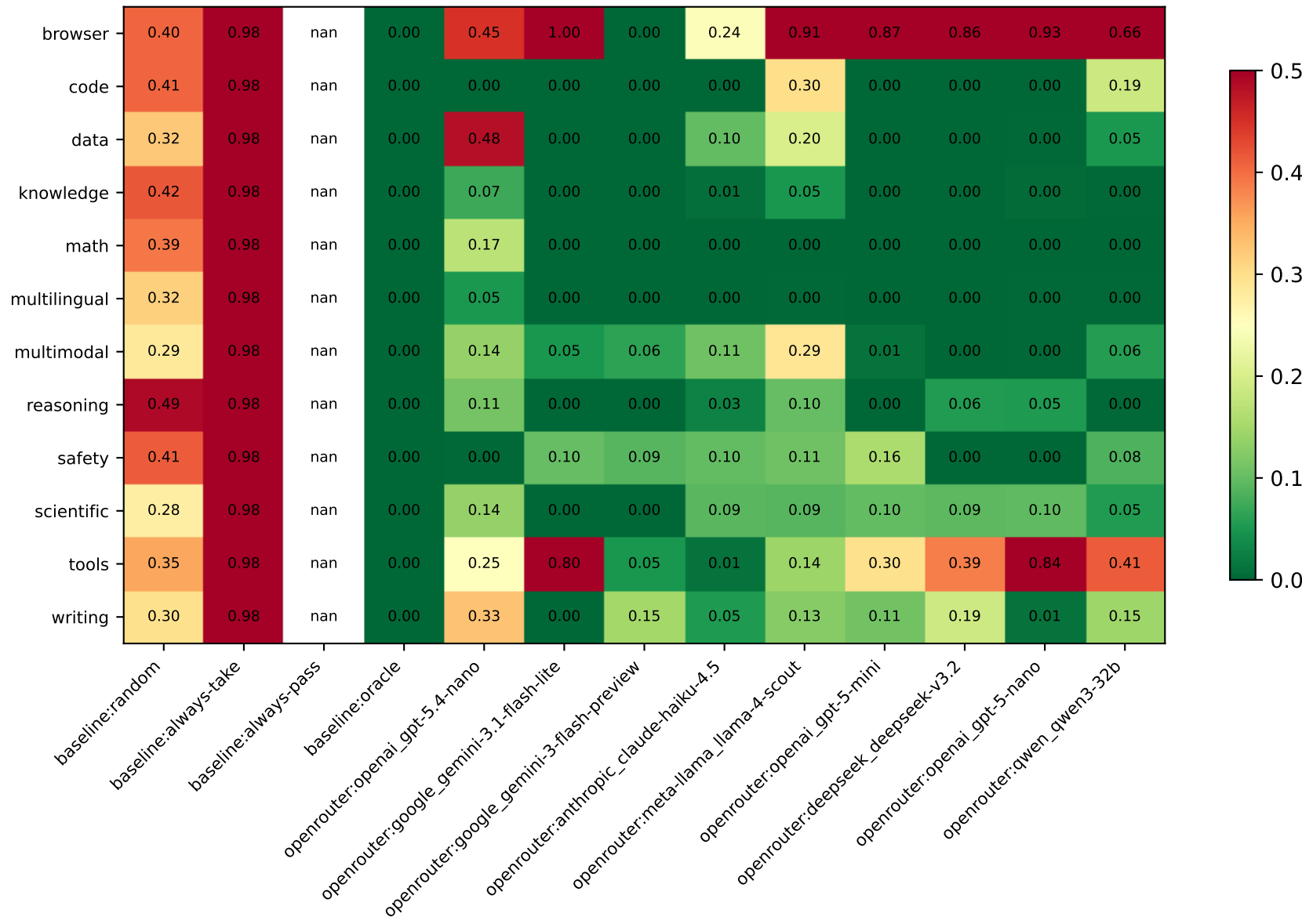
Per-family brier
