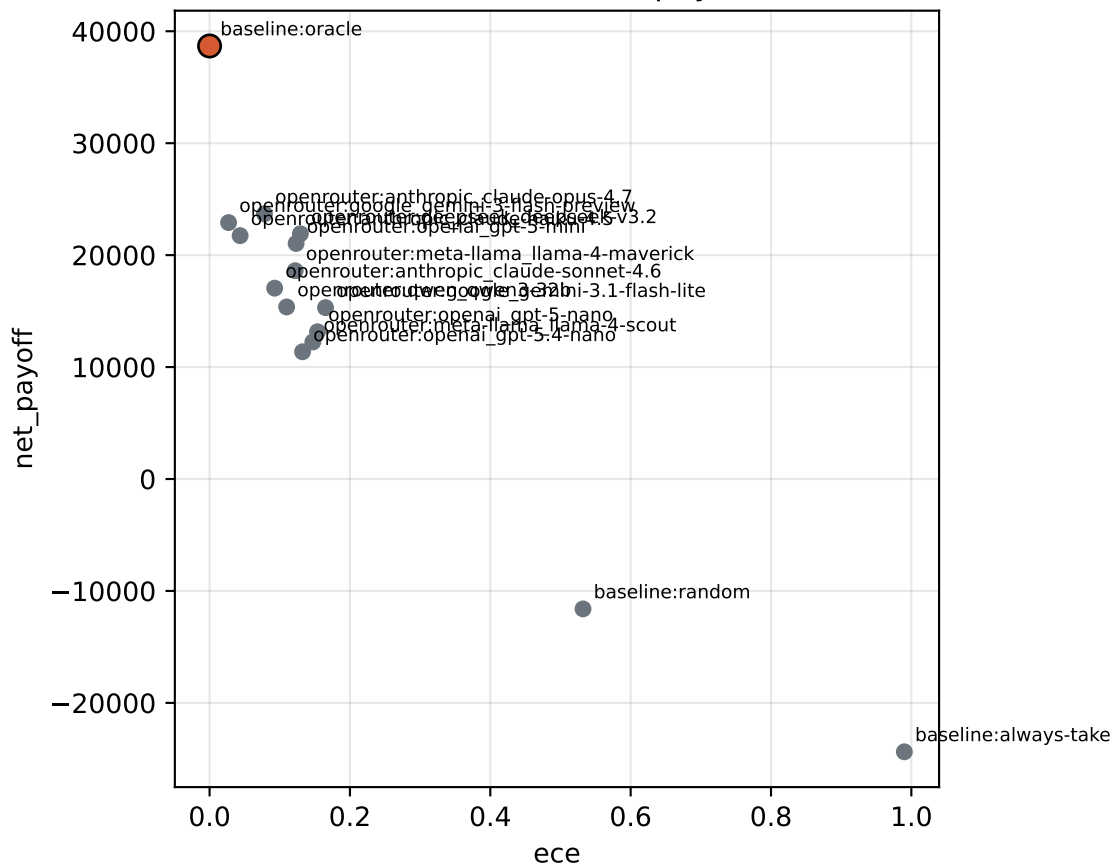
Pareto: ECE × net payoff
