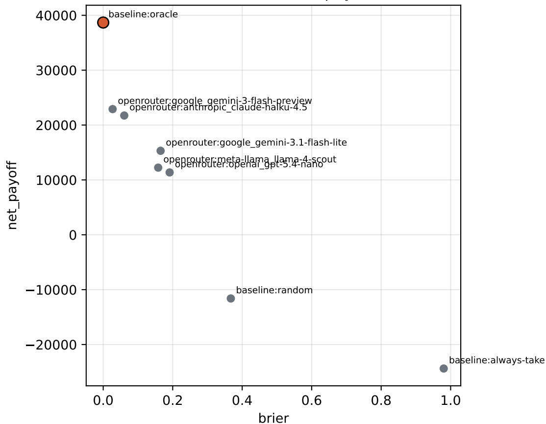
Pareto: Brier \times net payoff
