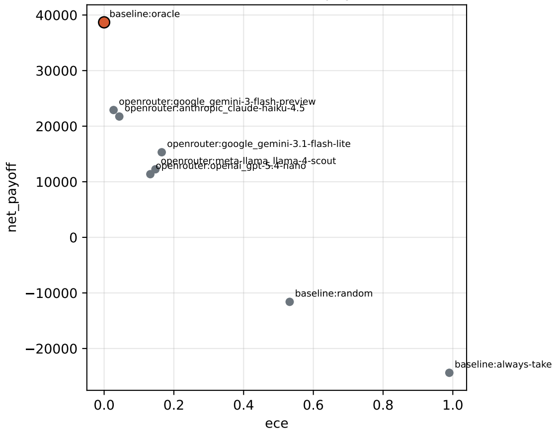
Pareto: ECE \times net payoff
