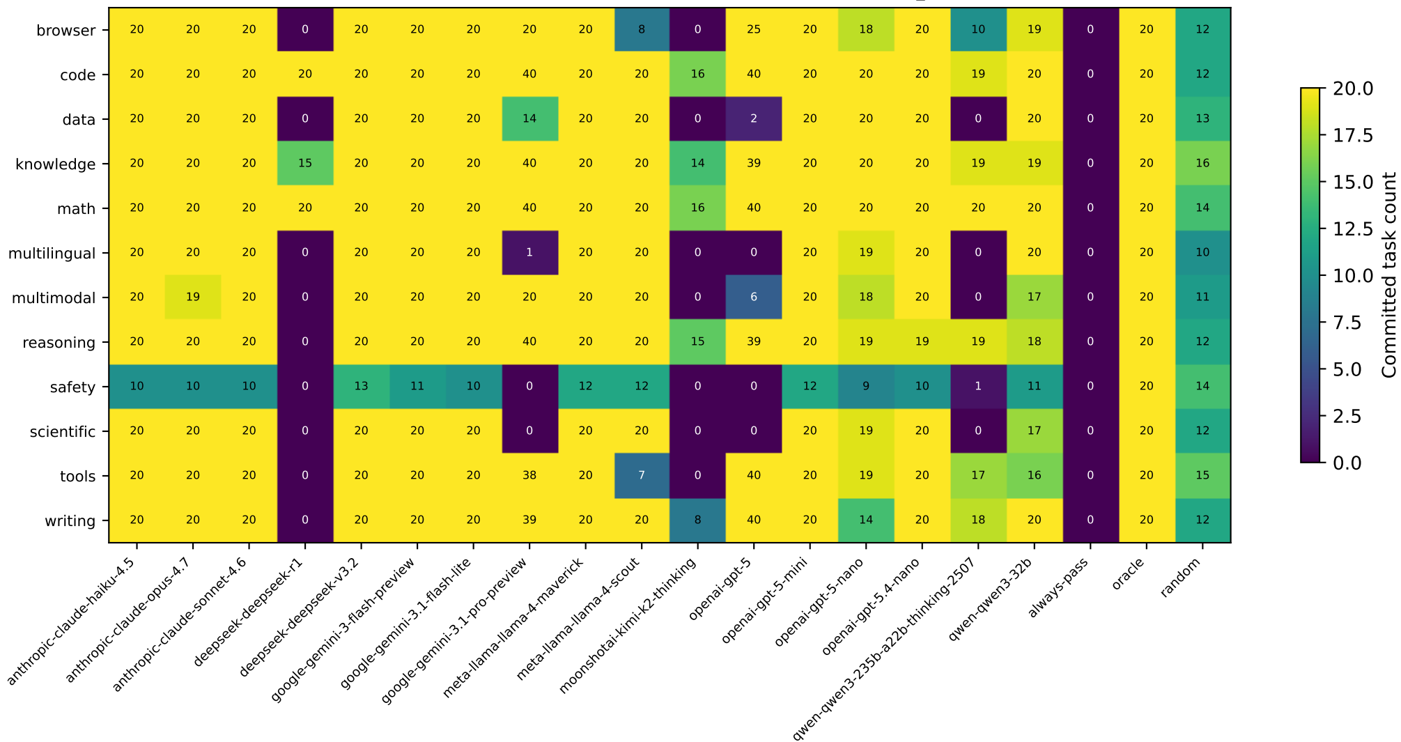
Per-family committed-task count. Zeros explain the NaNs in heatmap_accuracy.
