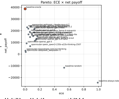
Figure 1: Pareto frontier on (ECE, P) . Points on the frontier in colour; dominated points in grey. Hypervolume against reference (ECE = -3NC) is
