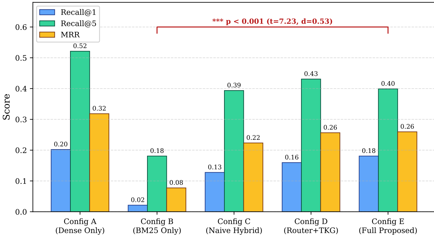
Figure 3: Component Ablation Benchmark across 188 Industrial Queries
