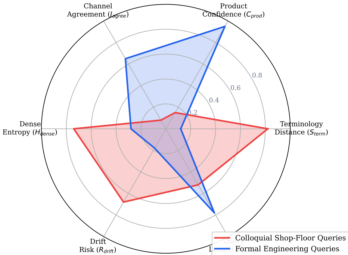
Figure 4: 6D Query Feature Space \Phi(q) Profile Comparison
