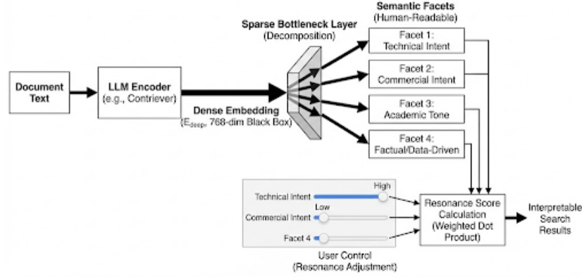
Figure 1: The ISR Architecture. Document text is processed by a standard LLM encoder into an entangled dense embedding ( E_{deep} ). The ISR Sparse Bottleneck Layer decomposes this black box into isolated, human readable Semantic Facets. During retrieval, users adjust these facets via UI sliders (User Control), dynamically scaling the Resonance Score Calculation to produce interpretable search results.
