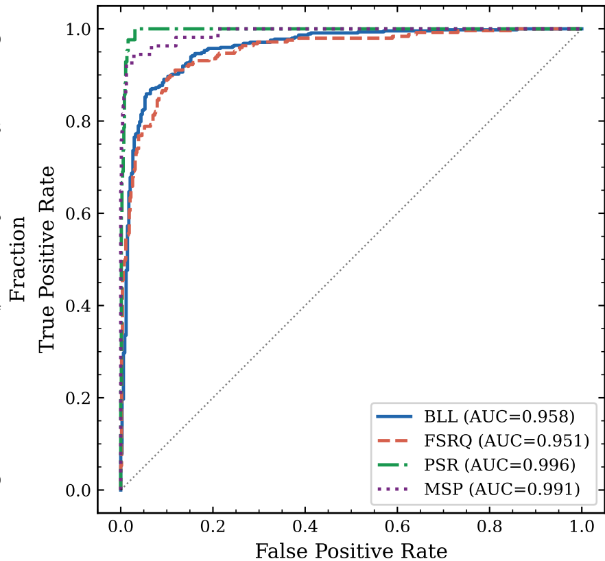
(b) One-vs-rest ROC (10-feat RF, test set)
