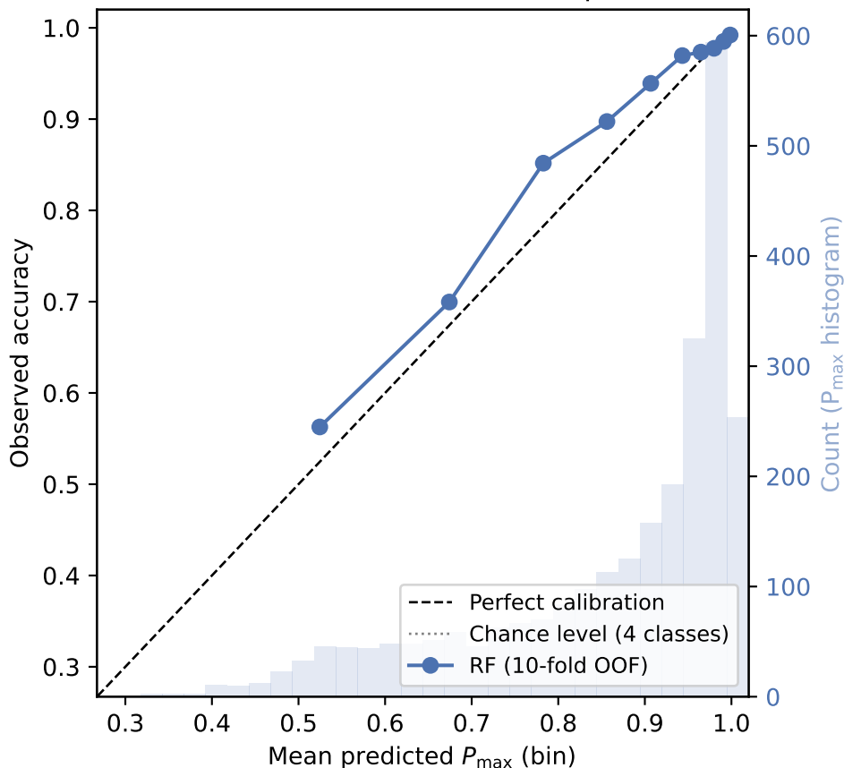
Calibration of RF posterior confidence (10-feature RF, 10-fold out-of-fold predictions)
