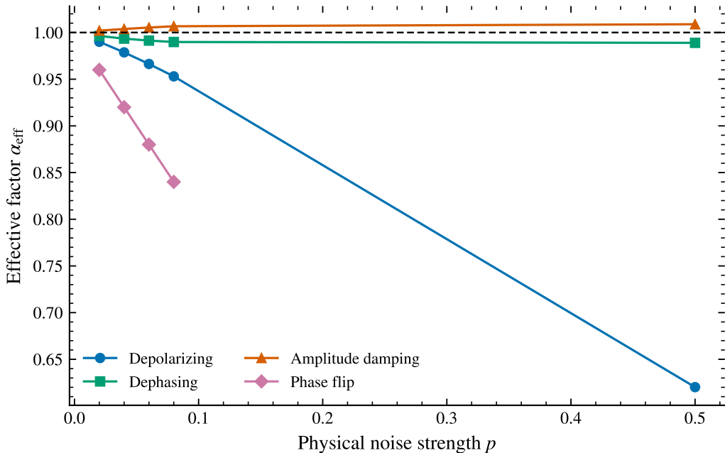
Effective exponential factor in R(s) = A\alpha^s
