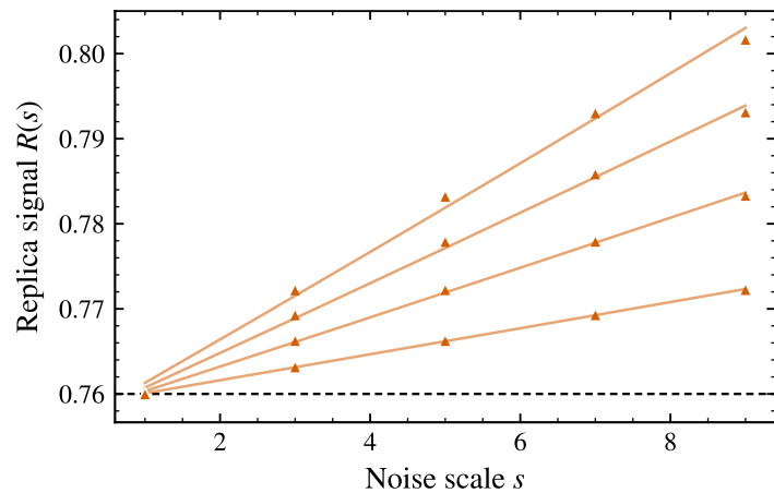
Amplitude damping (system, folded)
