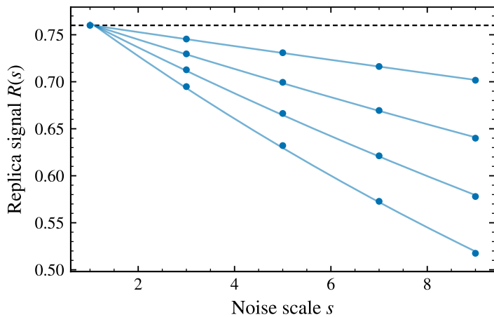
Depolarizing (system, folded)
