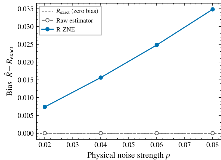
Depolarizing (system, folded)
