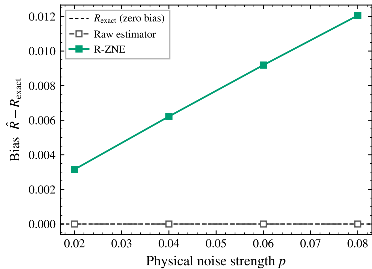
Amplitude damping (system, folded)
