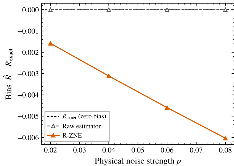
Amplitude damping (system, folded)
