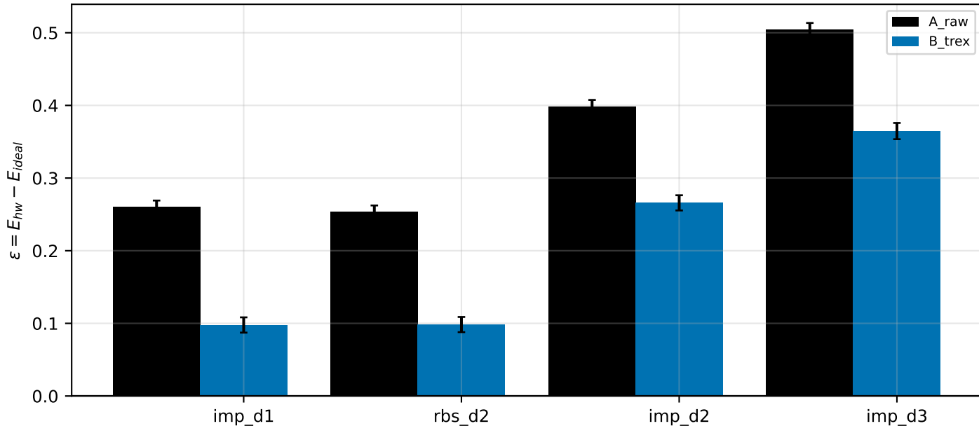
Hardware error relative to each circuit's own noiseless energy
