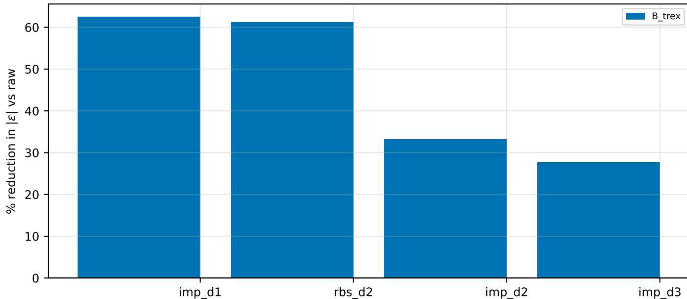
Mitigation-induced error reduction (negative means worse)
