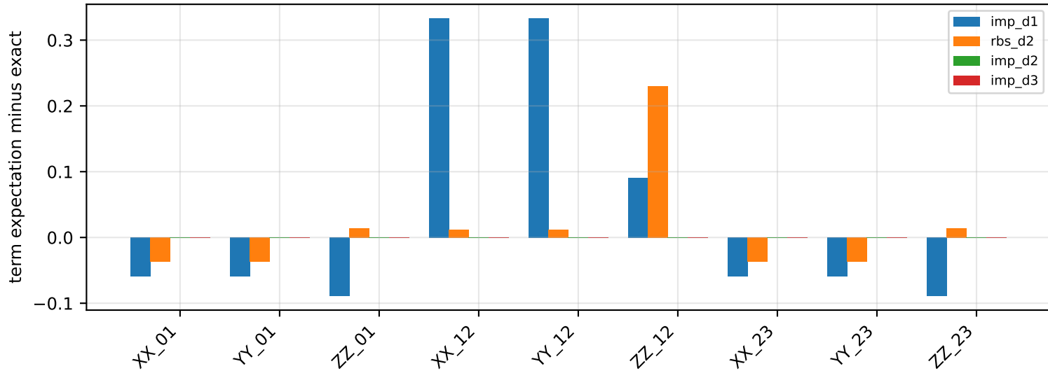
Ideal term-by-term deviation from the exact ground state
