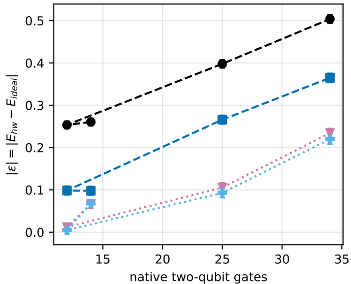
Exploratory: hardware error vs circuit cost (3 heterogeneous circuits)
