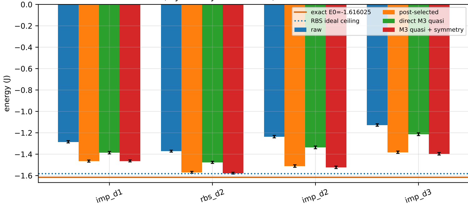
Raw, symmetry-conditioned, and M3 estimators
