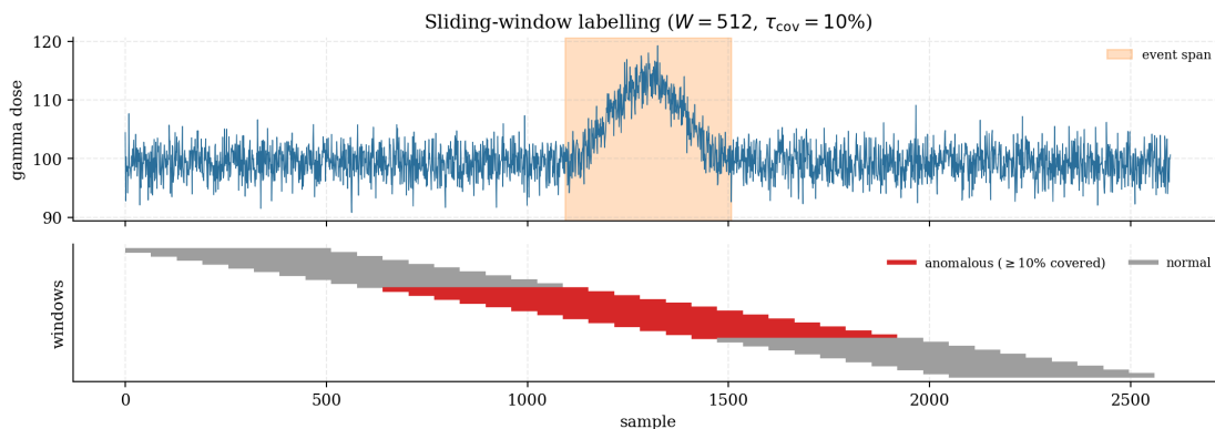
Figure 5.1. Sliding-window labelling on a fragment containing one event (orange span, top). Each bar (bottom) is one 512-sample window; a window is labelled anomalous (red) when at least \tau_{\text{cov}} = 10\% of its samples fall inside the event, and Normal (grey) otherwise.
