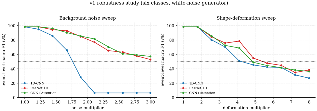
Figure 6.3. Robustness. Event-level macro F_1 vs background-noise multiplier (left) and vs shape-deformation multiplier (right).
