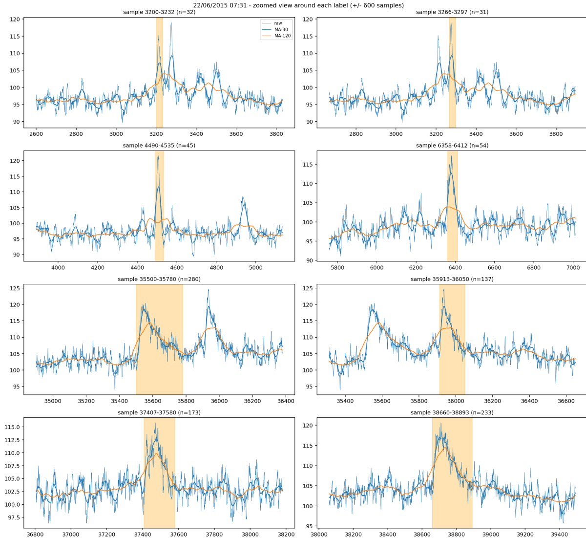
Figure 9.2. Zoomed view around each of the eight hand-labelled events in June 2015 ( \pm 600 samples of context). The orange band marks the labelled interval. The diversity of the events is visible: the first four are very short (30–55 samples) sharp spikes; the last four are longer (138–281 samples), with a mix of bell and asymmetric shapes. Note that on the June recording the labels sit on a slowly drifting baseline, illustrating why the per-event amplitude has to be measured against a local moving-average baseline rather than the global mean.
