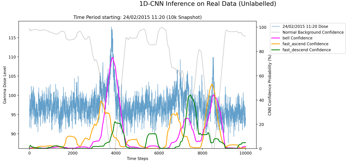
Figure 9.3. v2 1D-CNN inference on the first month of real 2015 data, first 10 000 samples. Blue: raw gamma dose. Grey: smoothed Normal Background confidence. Coloured curves: the three anomaly classes. Compared to the v1 version of this plot (fig. 7.1, top panel) the background confidence is now near 100% throughout the quiet regions and only drops where the raw signal contains a visible bump. The labelled Fevereiro event around sample 3 500 is recovered with high confidence as a bell/fast_ascend mixture.
