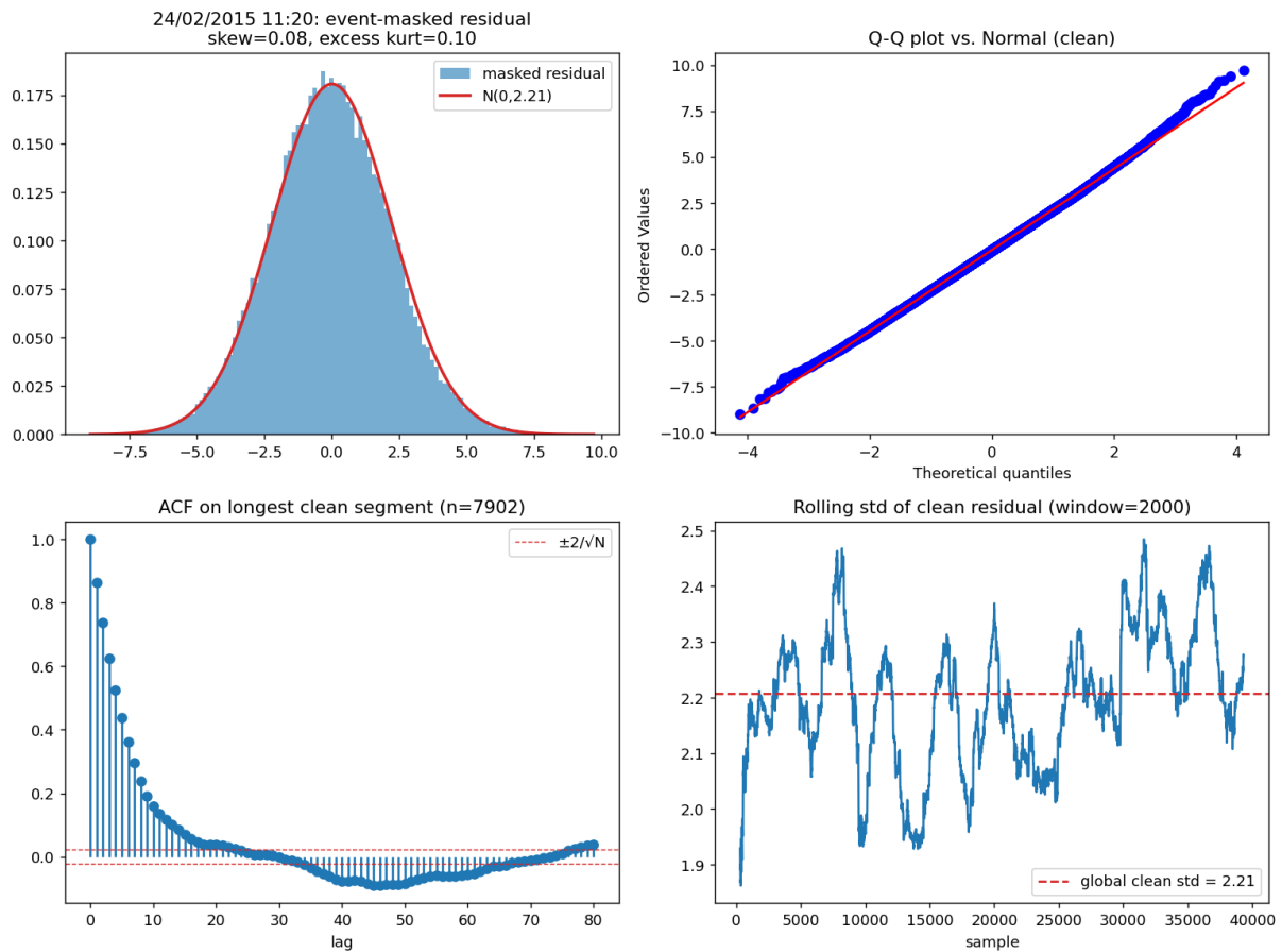
Figure 8.1. Diagnostics on the masked residual of February 2015 (clean fraction 93%). Top-left: histogram, near-perfectly fit by \mathcal{N}(0, 2.21) (red). Top-right: Q-Q plot vs. Normal, on the diagonal. Bottom-left: autocorrelation function on the longest contiguous clean segment — \text{ACF}(1) = 0.864 , decaying smoothly to zero by lag \sim 30 . Bottom-right: rolling-window standard deviation, stationary around the global value. The marginal distribution agrees with the IID-Gaussian assumption of eq. (3.2); the autocorrelation does not.
