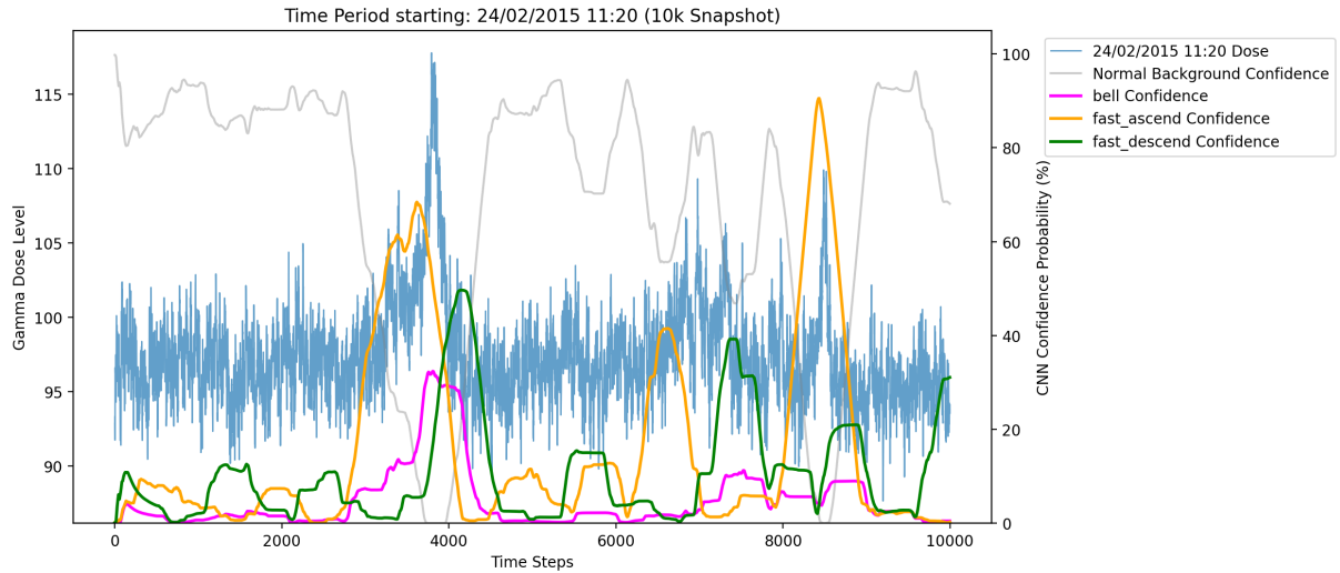
Figure 9.5. v2 CNN+Attention inference on the same window. The degenerate single-class collapse described in section 7.1 (the entire window pinned to M at \sim 100\% confidence) does not recur: the model sits on Normal Background between events and produces a clear fast_ascend response at the labelled event around sample 3 500.
