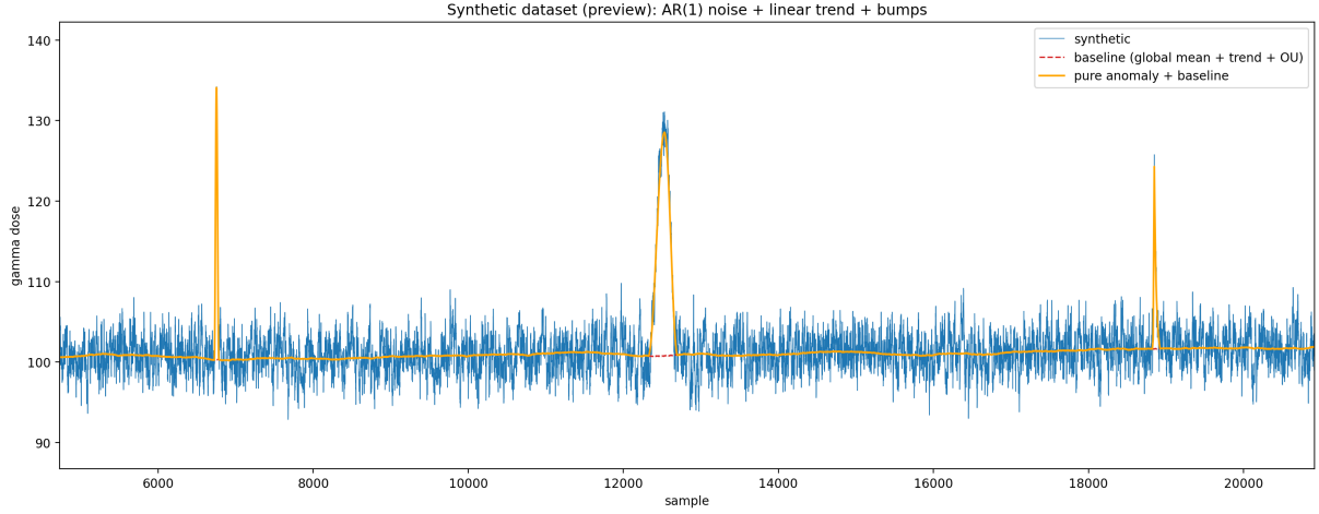
Figure 9.1. \sim 15\,000 -sample window from the v2 synthetic dataset. The blue trace is the synthetic signal (AR(1) noise on a tuned OU baseline); the orange trace is the pure injected anomaly pattern added on top of the baseline; the dashed grey line is the instantaneous baseline. Three injected events are visible in this window, at the v2 density of \sim 1.5 / 10,000 samples and with peak amplitudes drawn from the log-uniform [15, 40] range.
