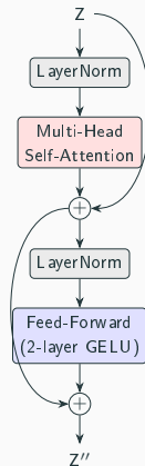
Pre-LN Transformer encoder block (residual around each sub-layer).
