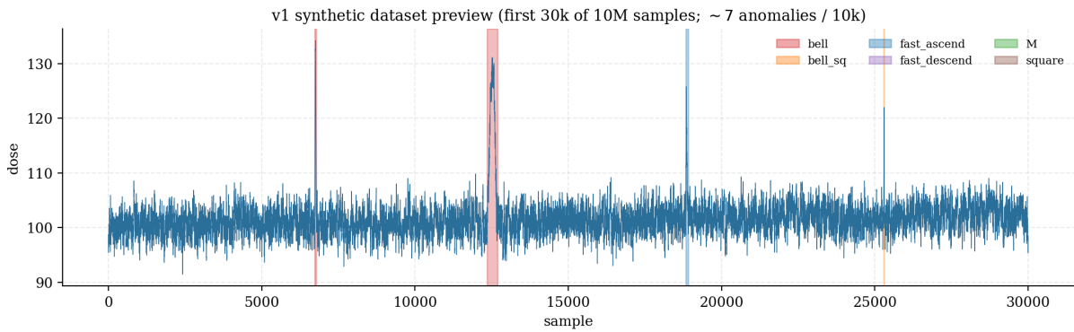
Figure 3.4. Excerpt of the synthetic dataset (first 30,000 of 10^7 samples). The gamma-dose signal (blue) fluctuates around \sim 100 counts; injected anomalies are highlighted and coloured by class (legend).
