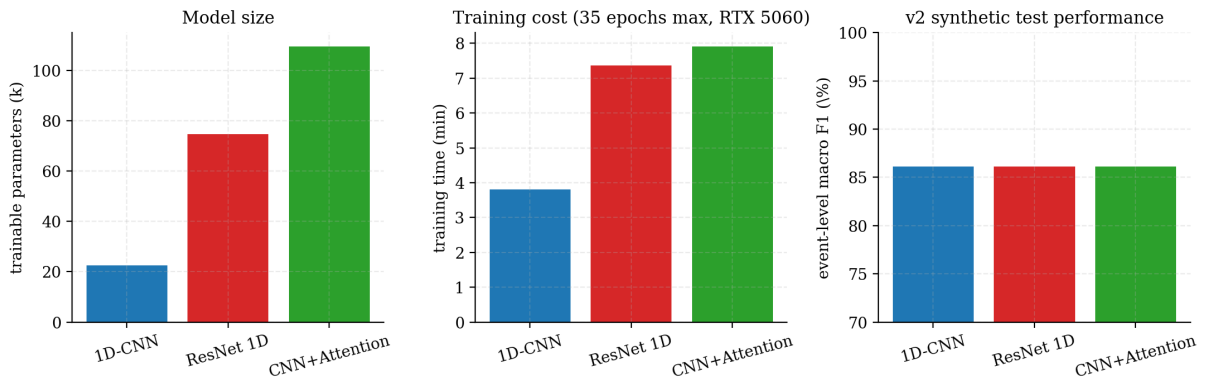
Figure 9.3. v2 cost–performance trade-off. Left: parameter count. Centre: total training time on a single RTX 5060 Laptop GPU (the 1D-CNN ran the full 35 epochs; the other two triggered early stopping after \sim 27 epochs). Right: event-level macro F1 on the synthetic test segment. Because the three networks converge to the same set of detected events on this segment, the F1 bars are equal.
