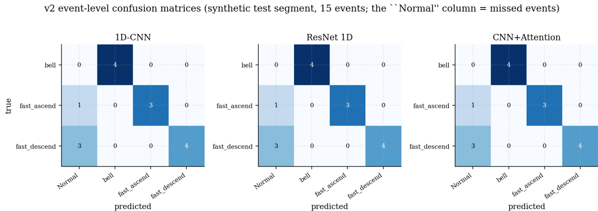
Figure 9.2. v2 event-level confusion matrices on the synthetic test segment. The leftmost column of each panel is the “missed event” column — a true event that has no overlapping prediction. All three models miss the same 4 events (out of 15): one fast_ascend and three fast_descend , all of them short events at the borderline duration of the detection threshold.
