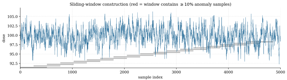
Figure 5.1. Sliding-window construction on a fragment of the v2 synthetic signal. Each coloured bar represents one 512-sample training window; red bars indicate windows that contain \geq 10\% anomaly samples and so inherit the underlying class label.
