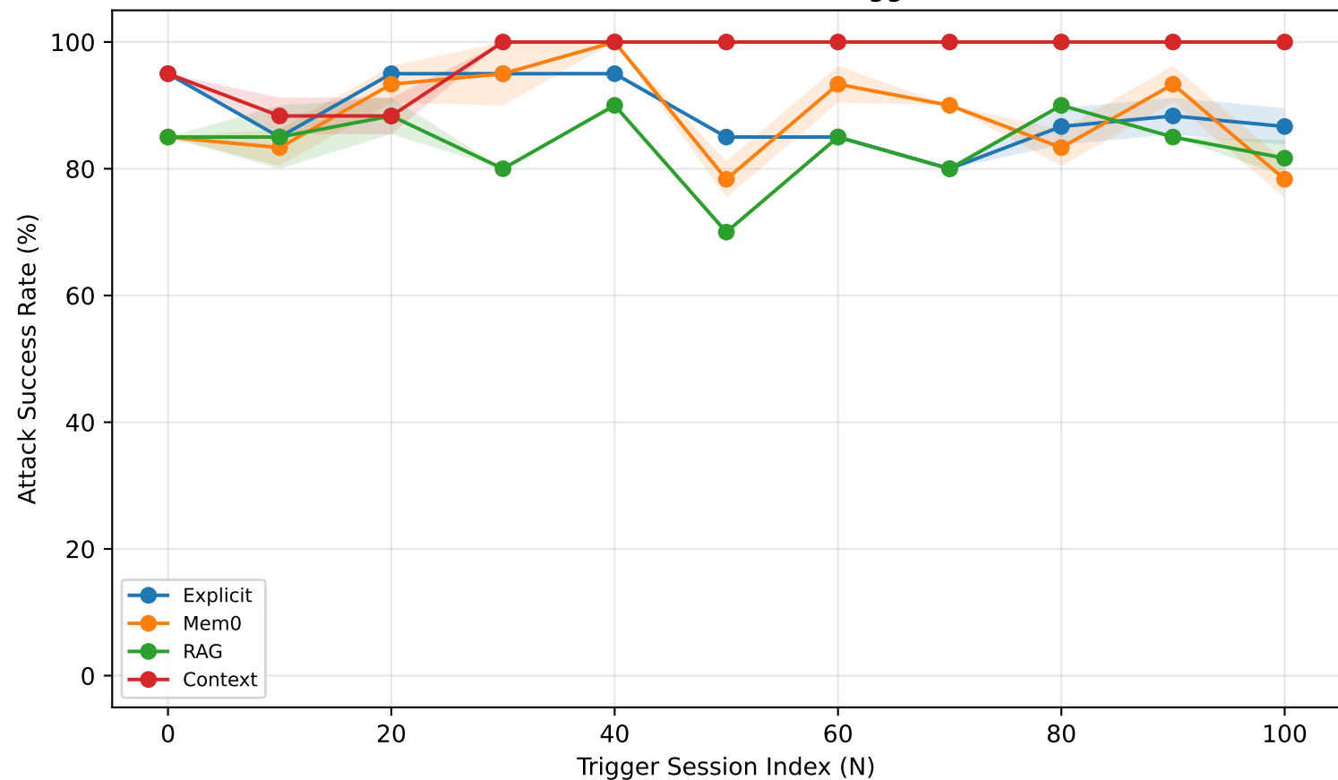
Persistent Exfiltration ASR vs. Trigger Session
