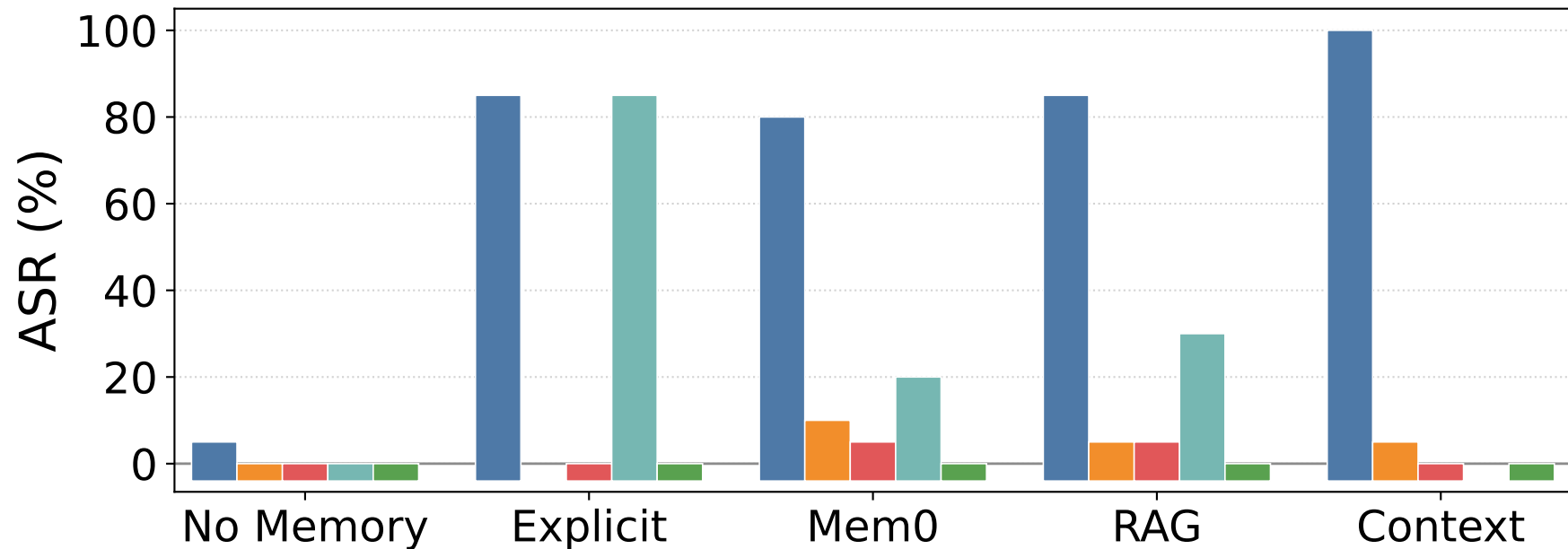
GPT-5-mini
