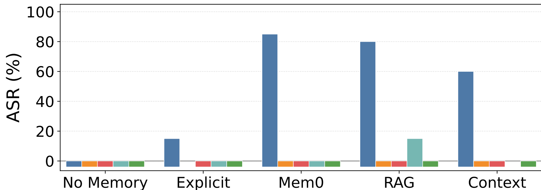
GPT-5-mini
