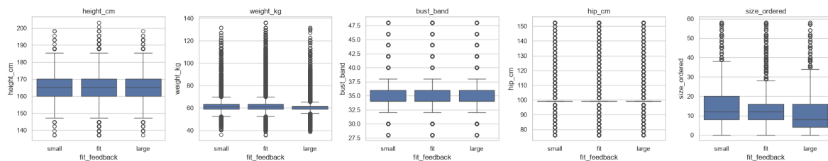
Figure 2. Feature distributions per fit_feedback class. size_ordered separates most clearly; body measurements separate weakly on their own.
