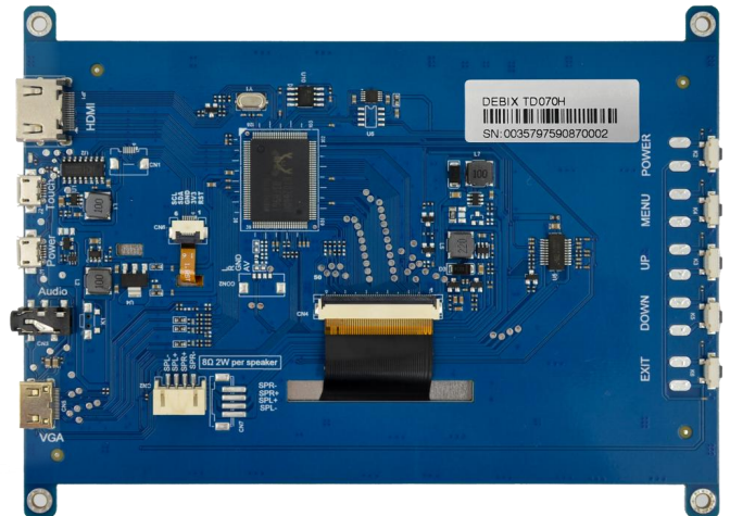
Back View of the DEBIX TD070H
