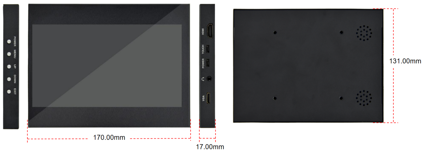
DEBIX TD070H-C (with AI alloy enclosure)
