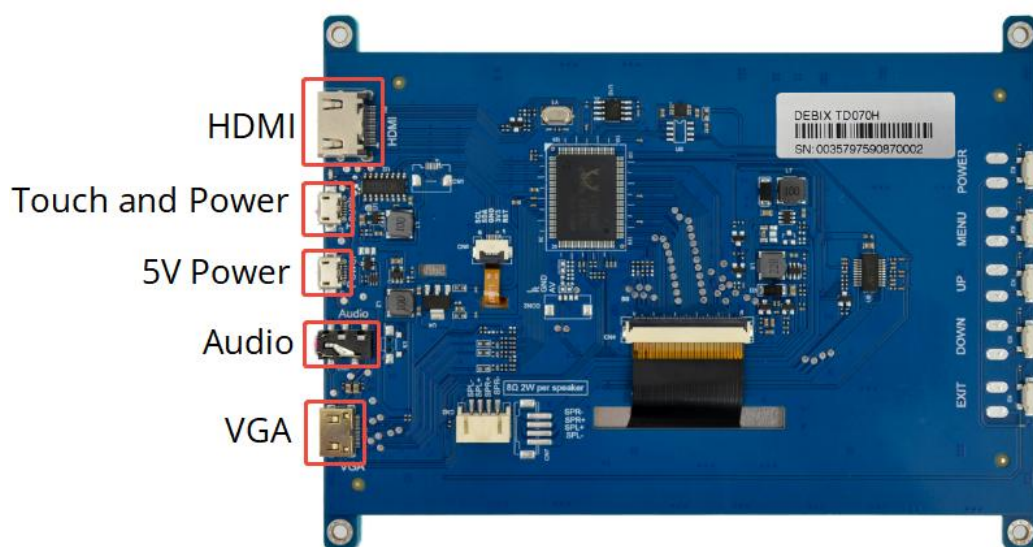
Figure 5 DEBIX TD070H Interfaces
