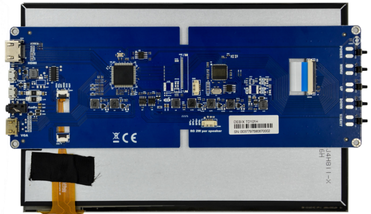
Back View of the DEBIX TD101H
