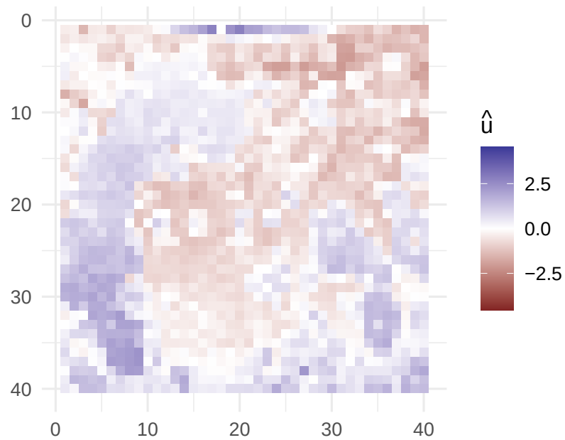
(c) Latent spatial effect: \hat{u}_k
