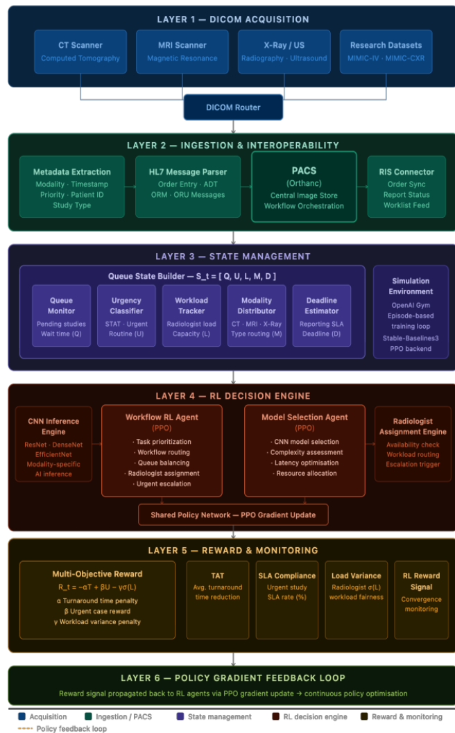
Figure 1a: System Architecture — RL Workflow Optimization Framework
