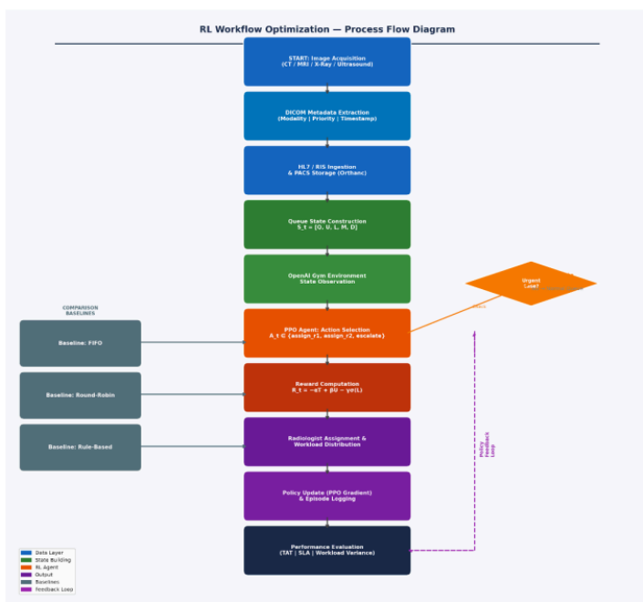
Figure 1b: RL Workflow Optimization — End-to-End Process Flow
